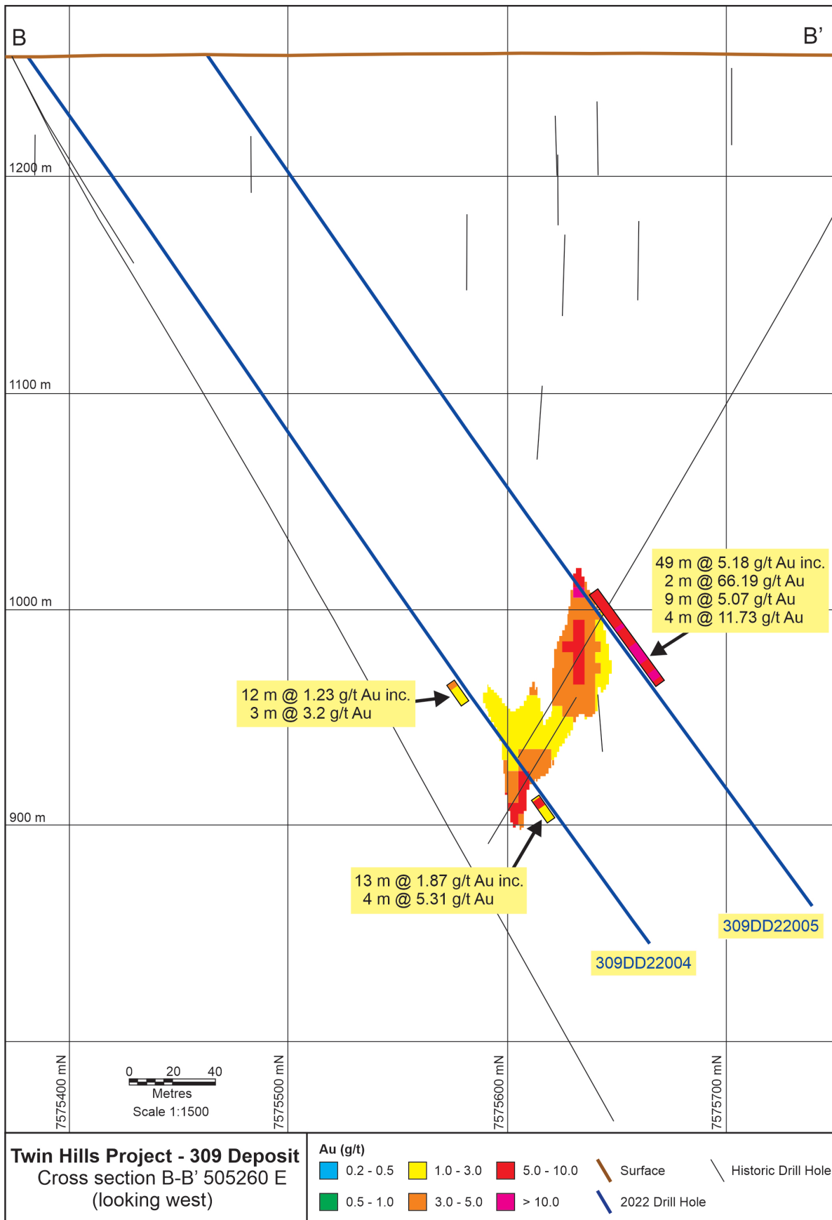
Figure 3. A cross-section showing assay results for 309DD22004 and 309DD22005. Only assays with a g*m value of > 10 are shown. Block model block grades from the 2022 resource update (ASX: GBZ release 2 February 2022) and historic drill holes are also shown.
