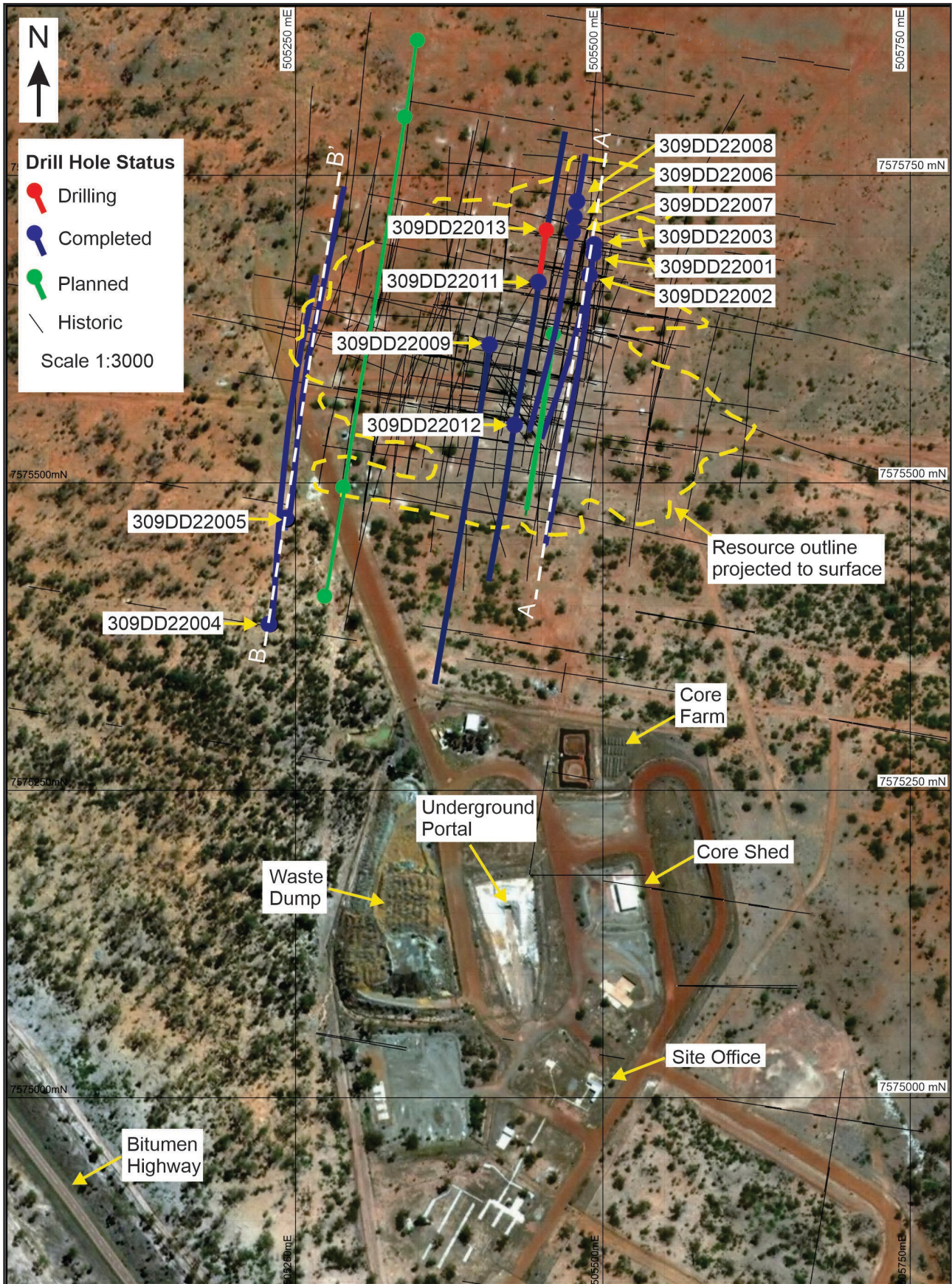
Figure 1: A map showing the location of recently completed and proposed drill holes at the 309 Deposit. Note the location of section line A-A' and B-B' for Figures 2 and 3 respectively. Also shown is established infrastructure, block model outline projected to surface and historic drill holes.
