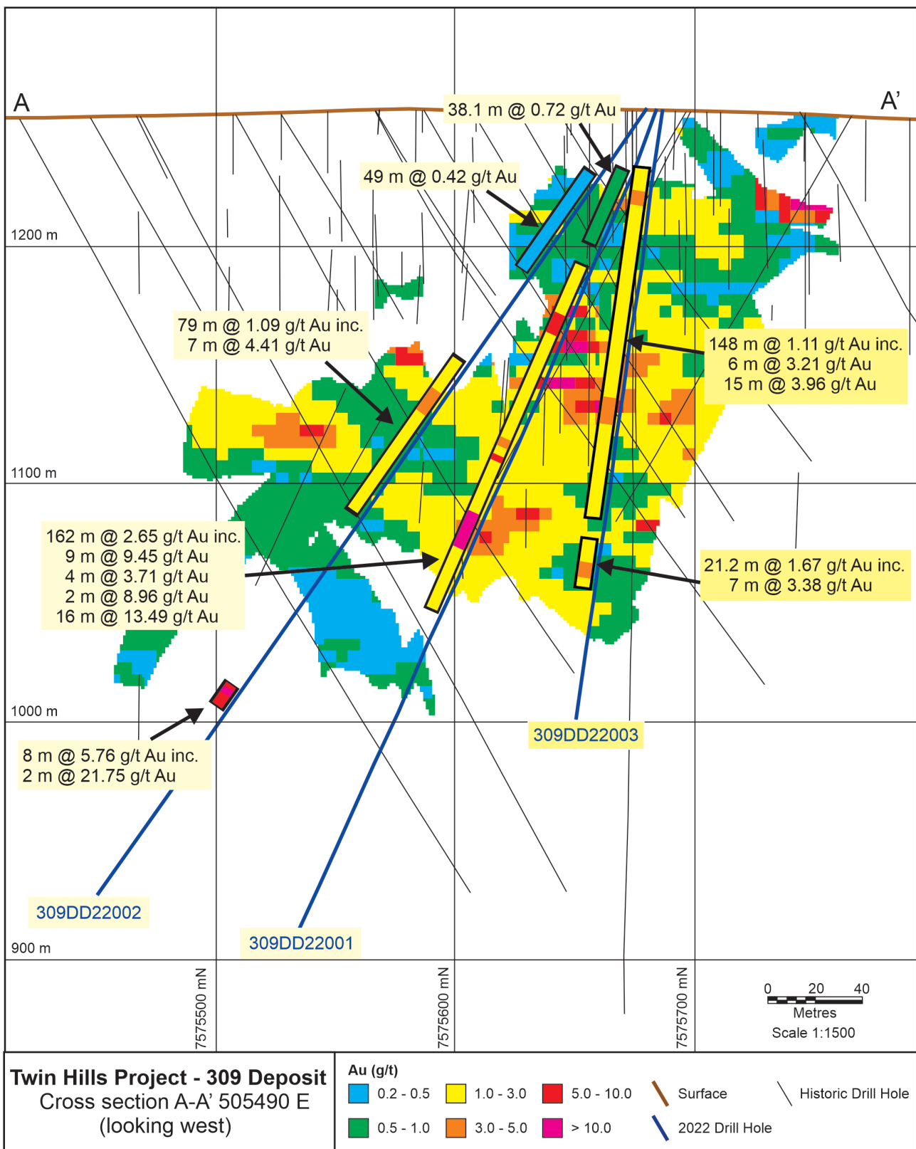
Figure 2: A cross-section showing assay results for drill hole 309DD22003. Also shown are assay results for 309DD22001 and 002 (ASX: GBZ release 6 April 2022). Only assays with a g*m value of > 10 are shown. Block model block grades from the 2022 resource update (ASX: GBZ release 2 February 2022) and historic drill holes are also shown.
