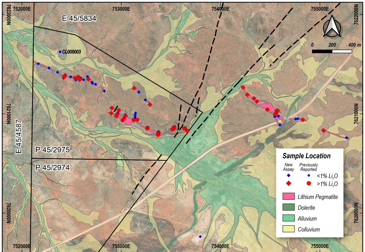
Figure 2 – Geology map showing the distribution of the lithium pegmatite. Also shown are the \text{Li}_2\text{O} values for all the samples collected and analysed, including results released previously 1 .
