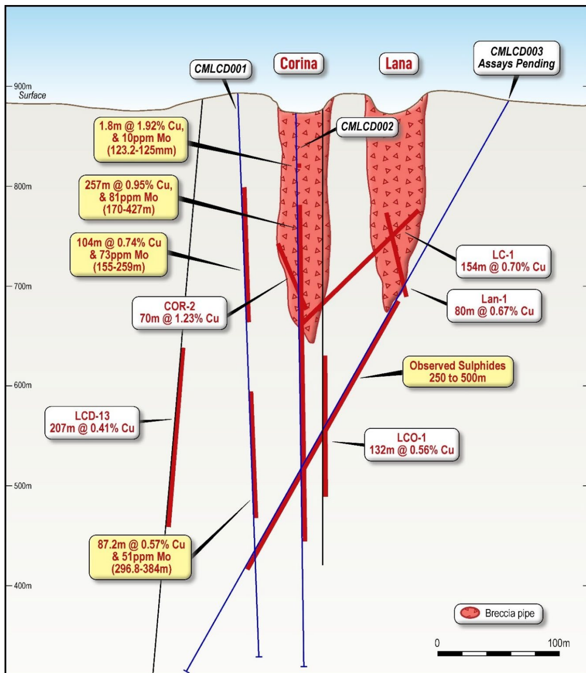
Figure 3: Long section view, looking west (section B-B') showing position of drillholes and targeted breccia units, section window +/- 100m.
