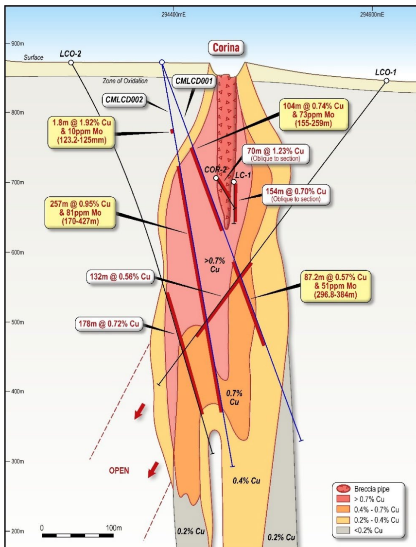
Figure 1: Sectional view looking northeast (section A – A') of Lana Corina with the location of drillholes CMLCD001 and CMLCD002 showing recent assay results, historical drill intercepts and copper grade contours, section window +/- 100m.
