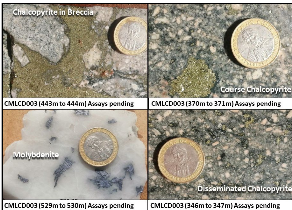
Figure 4: Visible mineralisation styles identified in drillcore from CMLCD003. Results for CMLDC003 are based on visual inspection only and have not been assayed
