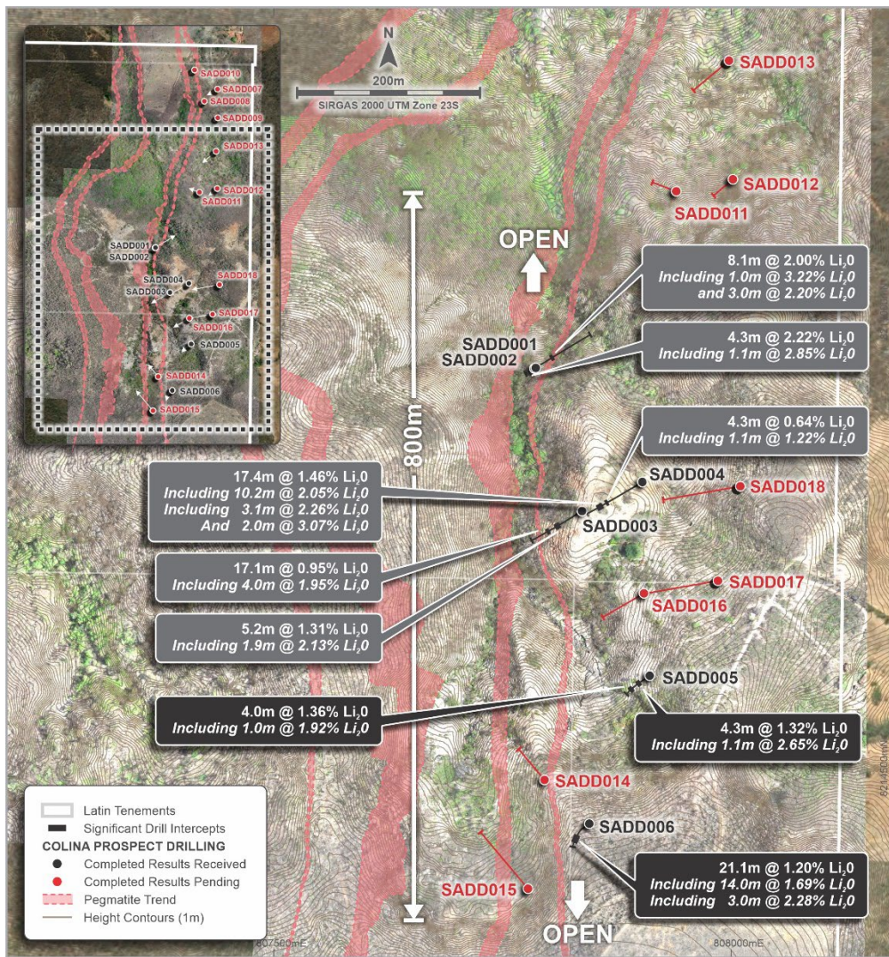
Figure 4: Colina Prospect area, showing completed drill collars and significant intersections 3 received to date
