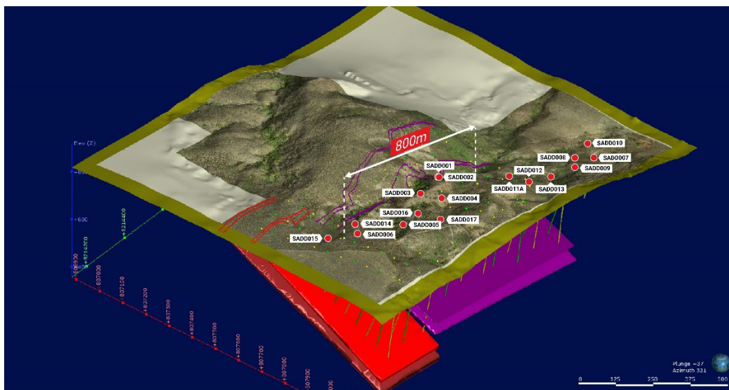
Figure 2: Oblique projection of the Colina Prospect area showing existing drill collars (red) and the planned (green/yellow) drill collars of the resource definition drilling campaign
