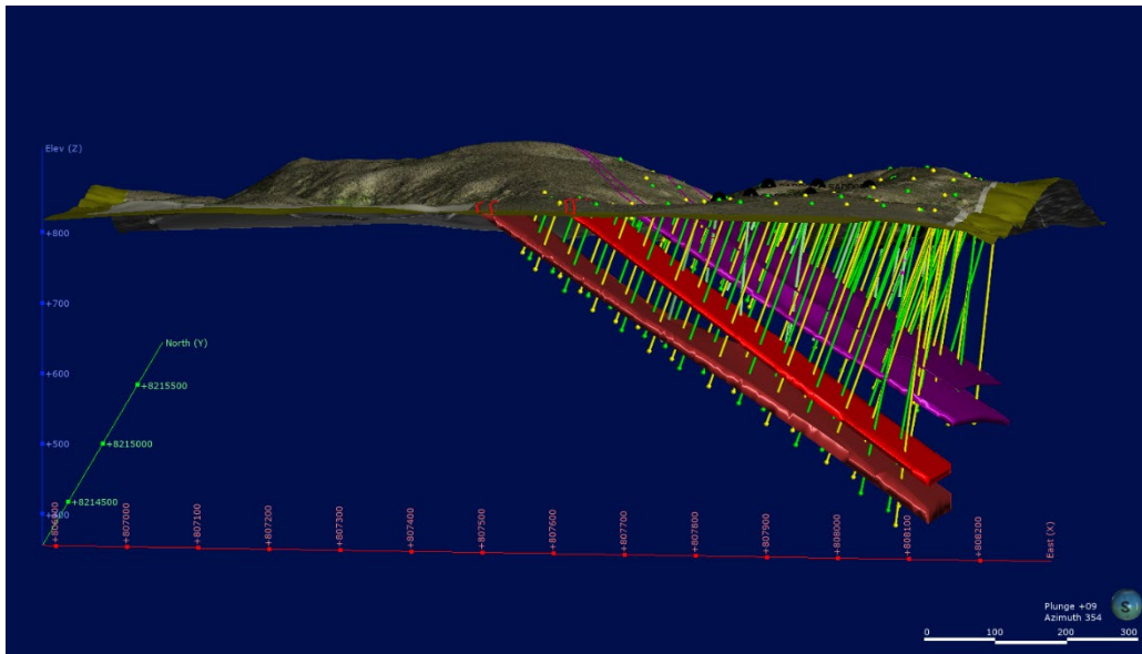
Figure 1: Oblique projection of the Colina Prospect area showing existing drill collars (black), and the planned (green/ yellow) drill collars of the resource definition drilling campaign
