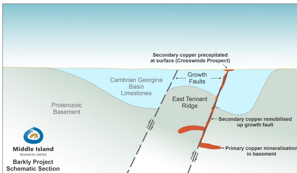
Figure 3 Crosswinds Copper Gold Project –Cross-section of interpreted setting
