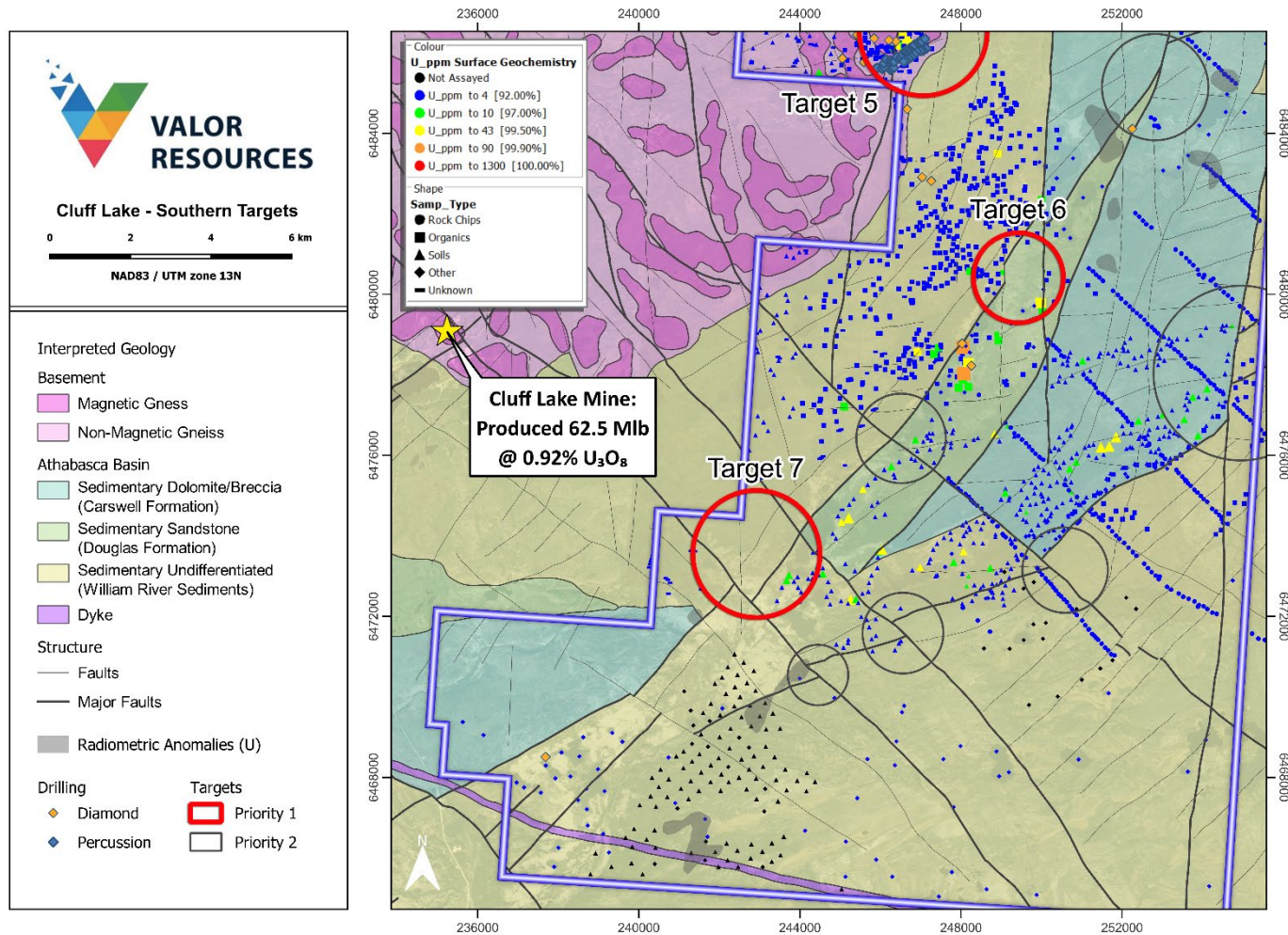
Figure 3: Cluff Lake Project – Southern Targets identified through historical data review and geophysical interpretation, showing historical surface sampling and drilling
