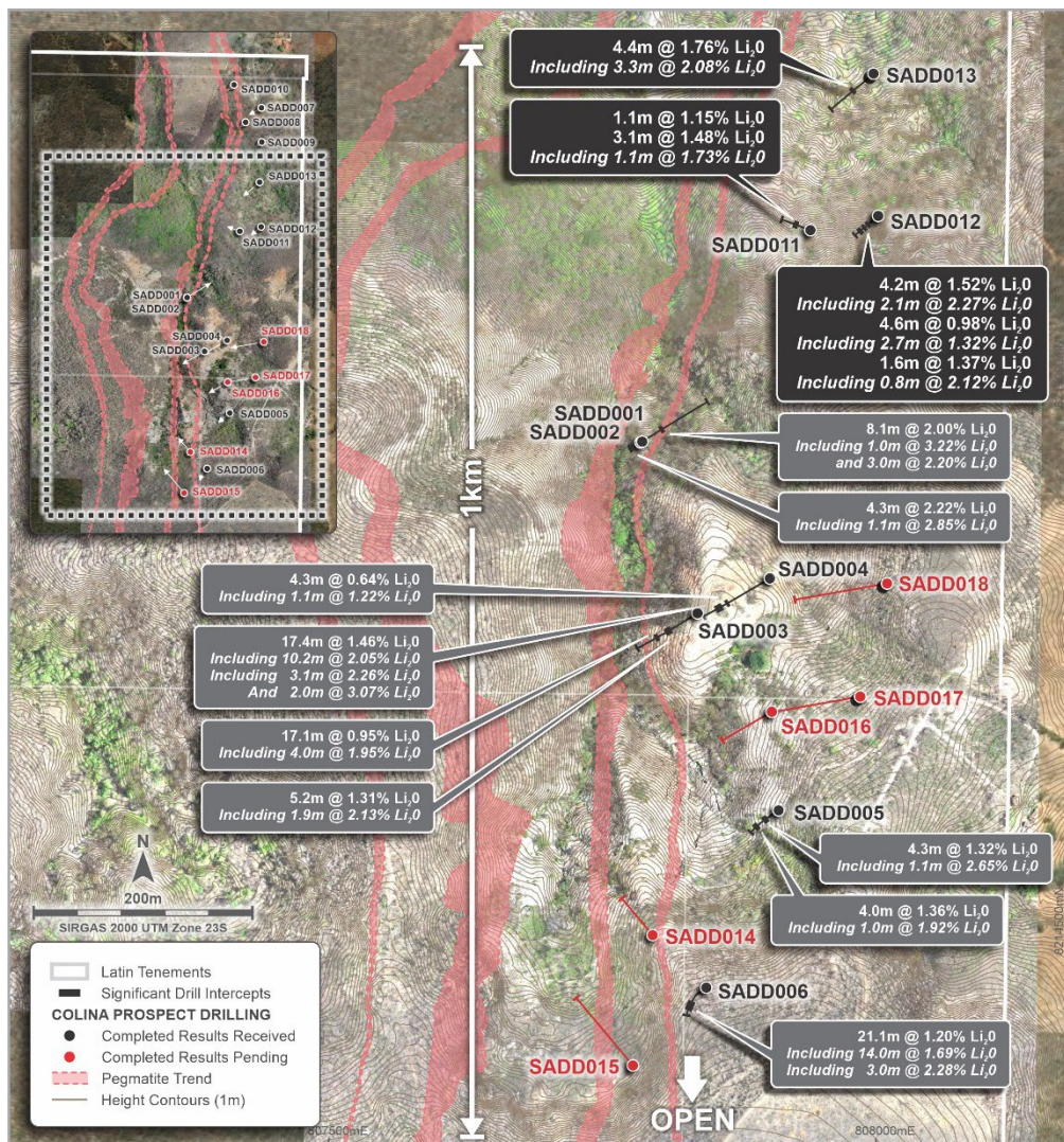
Figure 1: Colina Prospect area, showing completed drill collars 2 and significant intersections received to date
