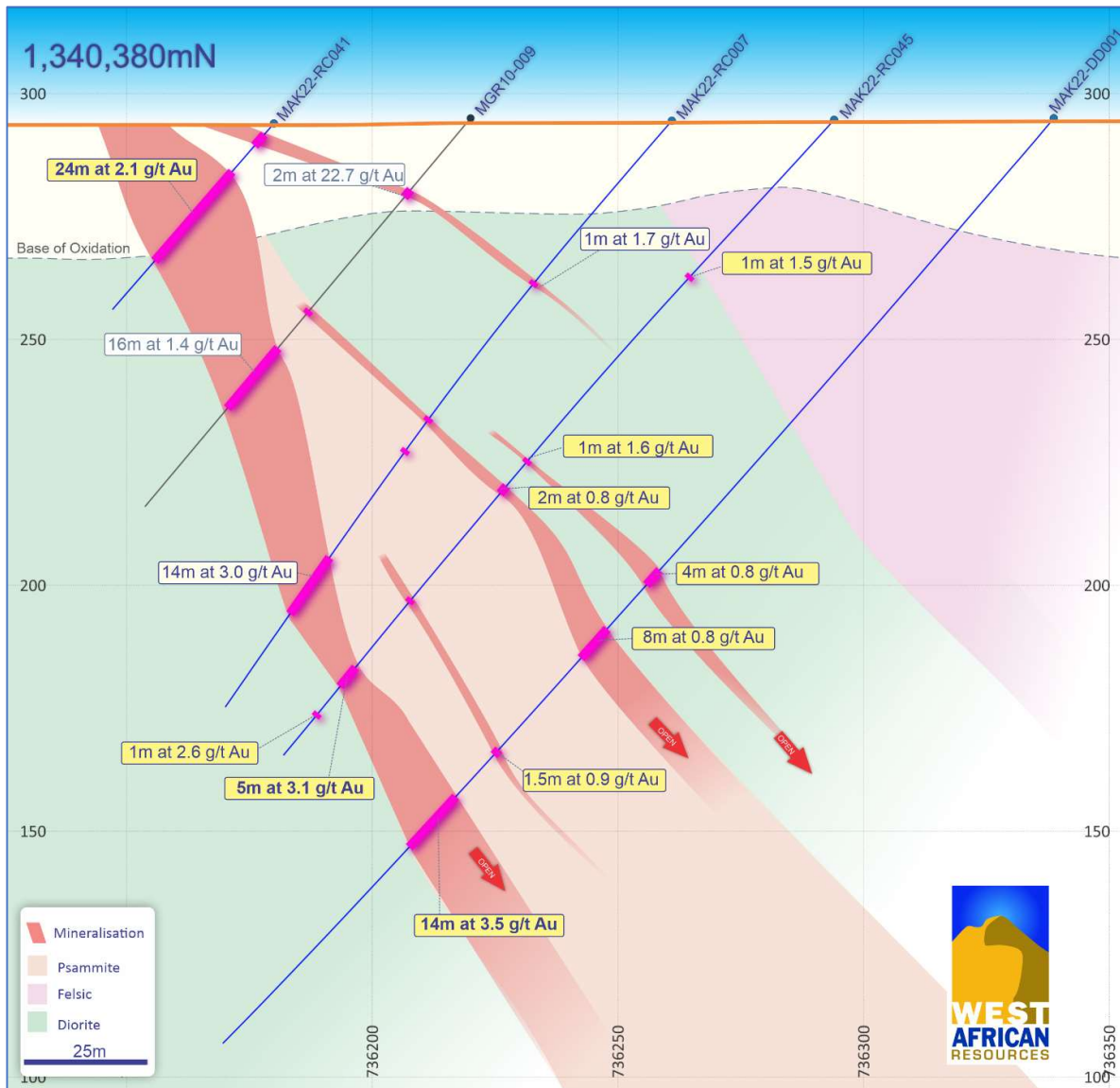
Figure 4: MV3 East cross-section 0330mN (Section A)
