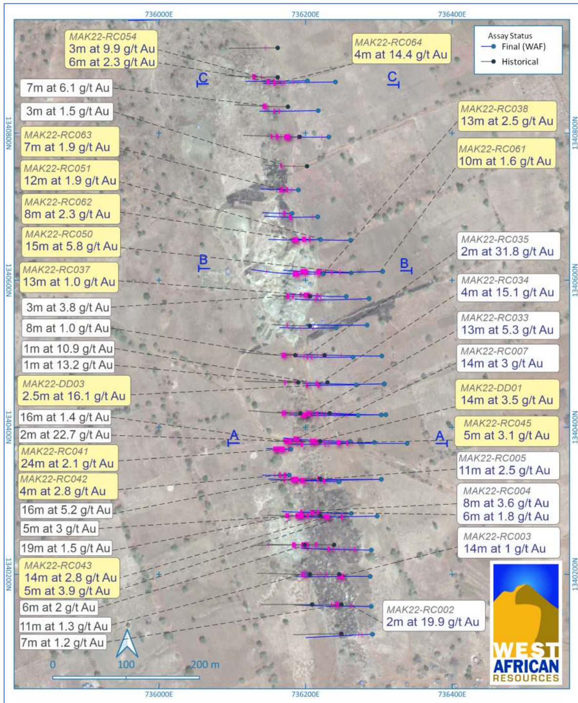
Figure 3: MV3 East Drillhole Location Plan
