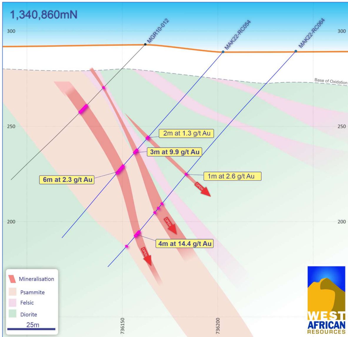
Figure 6: MV3 East cross-section 0420mN (Section C)
