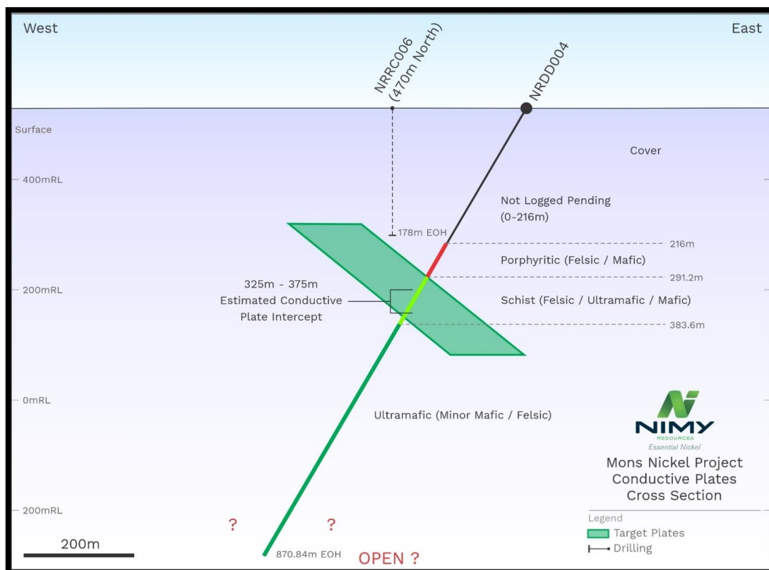
Figure 2 – Diamond Hole – NRDD004 – Cross section
