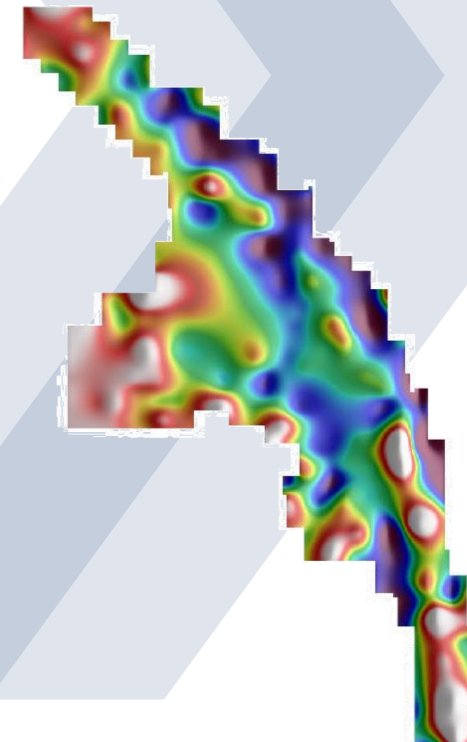
Regional Gravity
