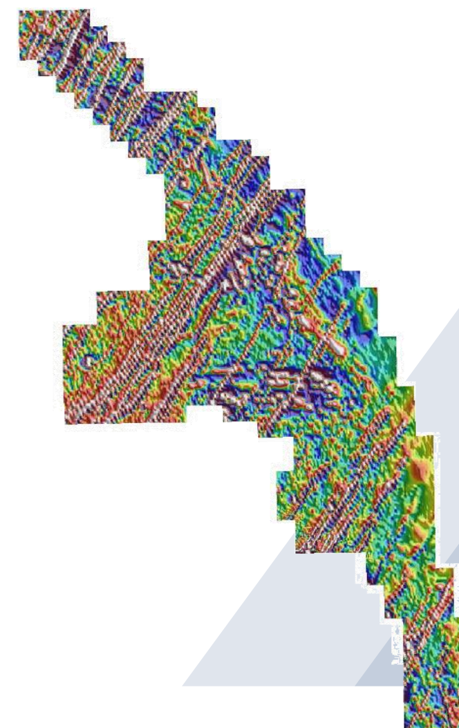
Magnetics RTP, 0.5 Vertical Derivative
