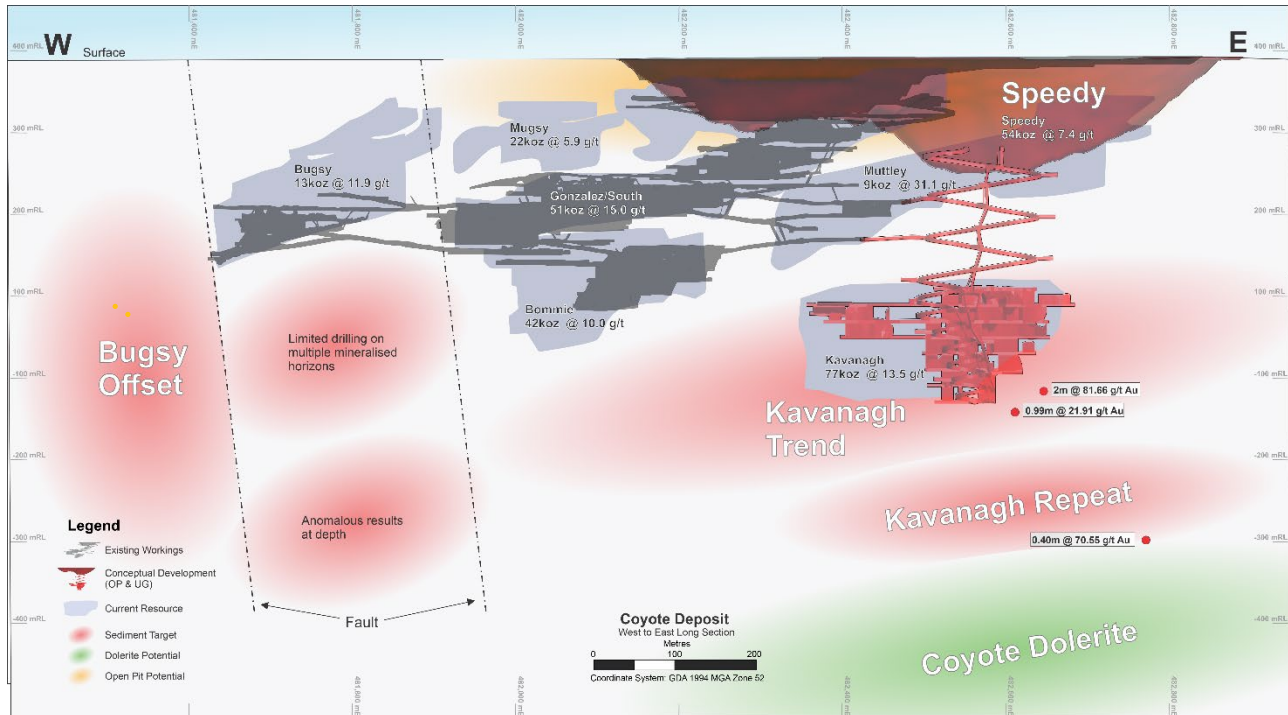
Figure 2: High priority, near-mine targets: Speedy open pit, Kavanagh Trend and Repeat, Coyote Dolerite and Bugsy Offset.
