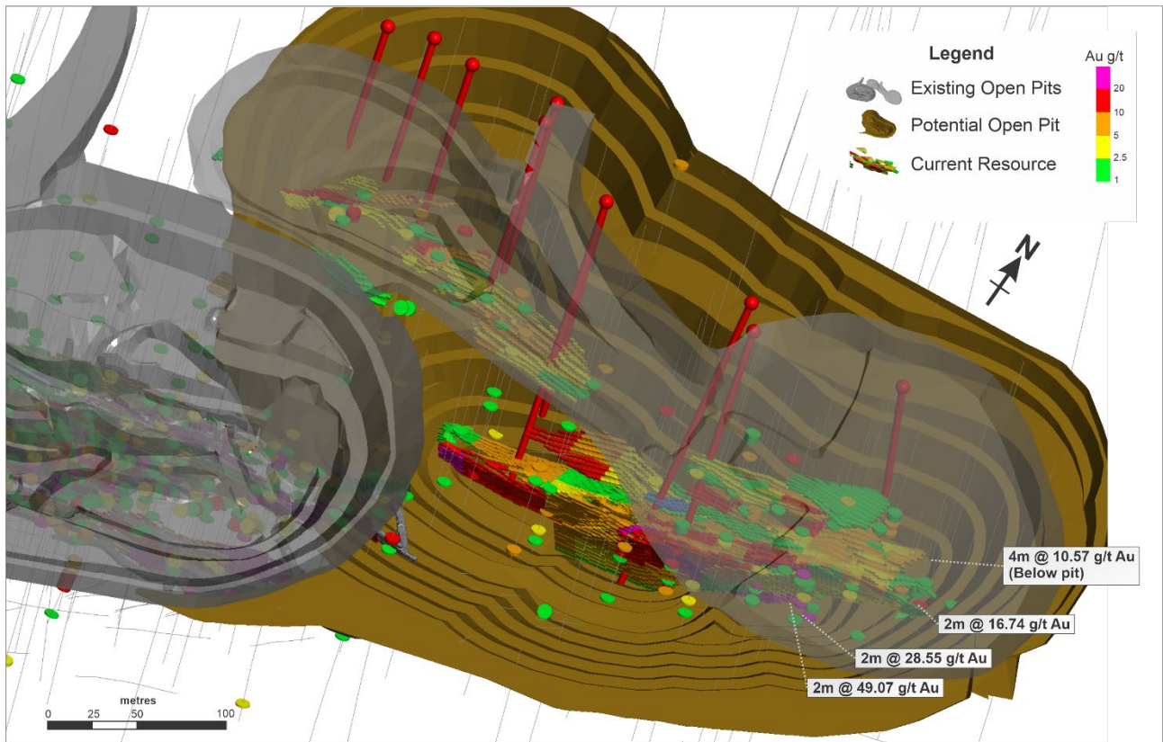
Figure 3: Oblique view looking NW of the current Resource with existing (grey) and the potential expanded (brown) open pit
