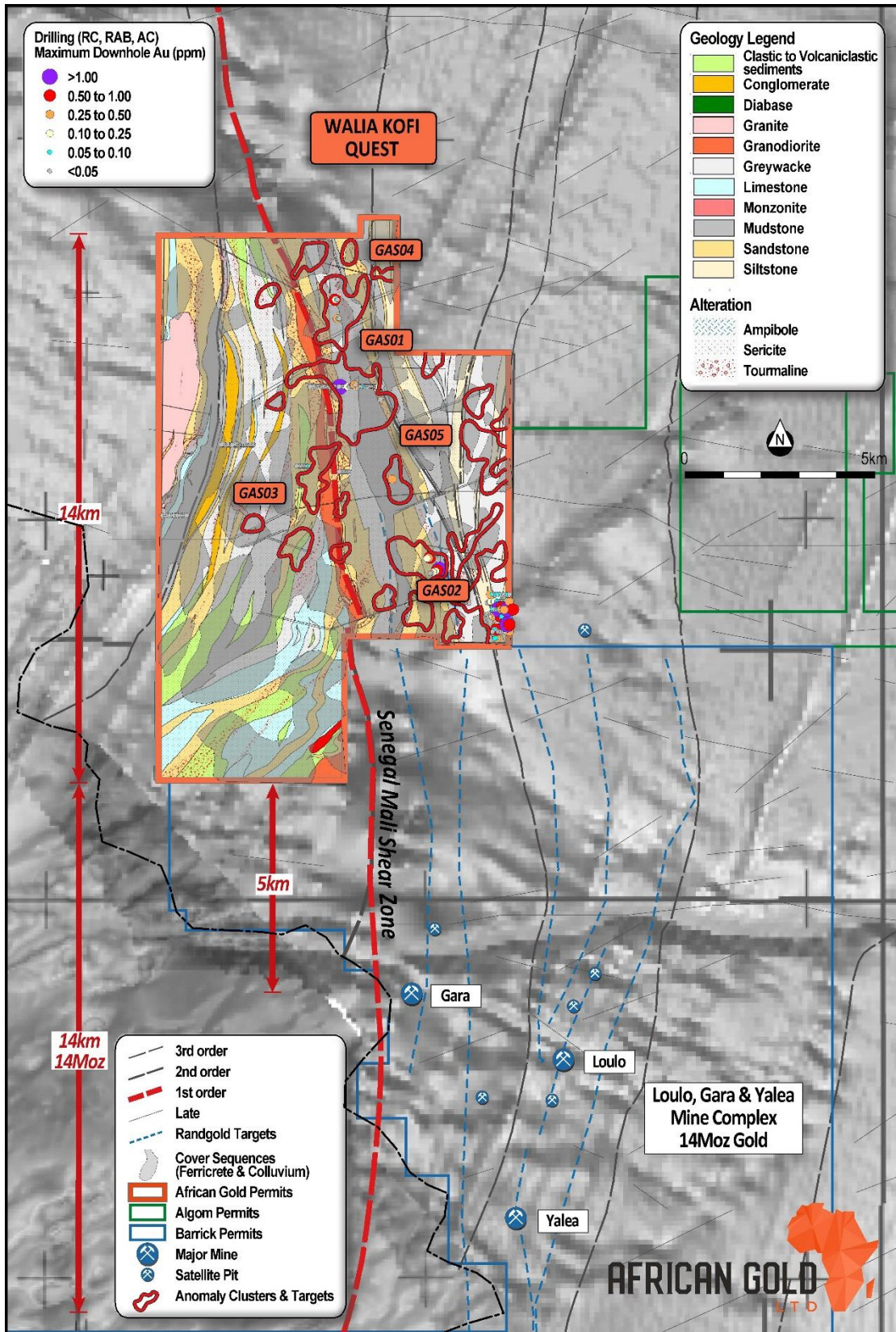
Figure 4: A1G's Walia Gold Project showing interpreted geology, SMSZ and identified higher order structures, major mines, deposits and prospects on a grey scale magnetic image. Also shown is extent of ferruginous and transported cover sequences with historical drill holes thematically mapped by maximum downhole gold grade. Priority targets for follow-up- also included.
