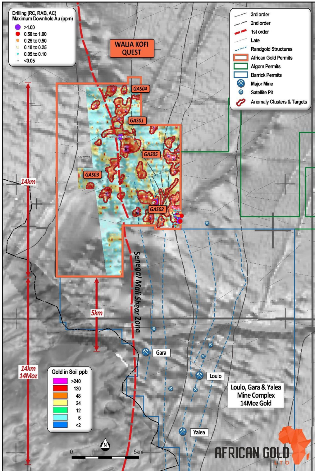
Figure 3: AIG's Walia Gold Project showing, major mines, deposits and prospects together with the SMSZ and interpreted higher order structures on grey scale airborne magnetic image. Results of gold in auger and soils are shown with historical (maximum down hole gold) and targets. Priority targets for follow-up RC drilling also included.
