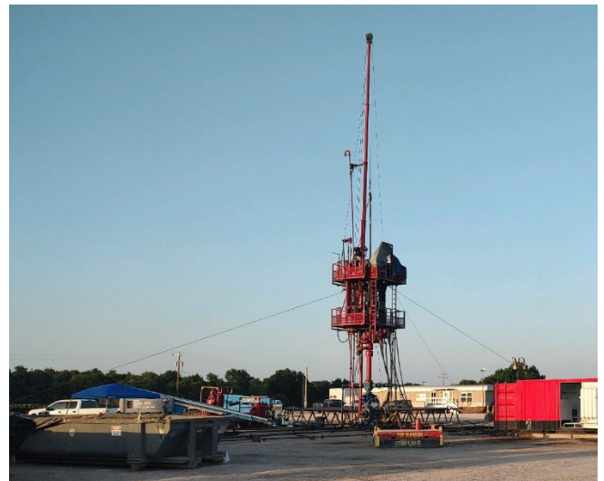
Figure 1. Snubbing unit on location at the Flames Well, Carter County, Oklahoma
