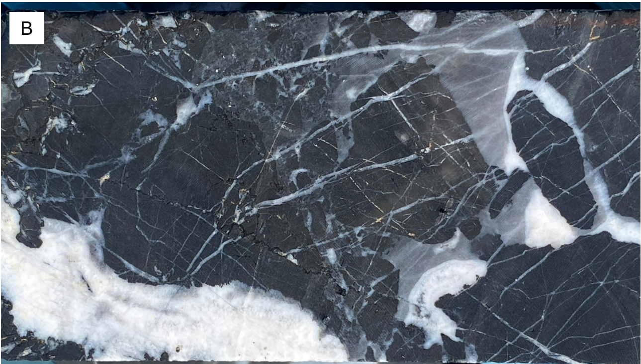
Figure 4: Photographs of drill core showing (A) Quartz-chalcedony-breccia fill hosted by milled matrix breccia at 121.9 m in 309DD22013. The interval assayed at 1.1 m @ 60.61 g/t Au from 121.7 m and (B) Multi-stage quartz-chalcedony veins and breccia fill at 262.6 m in 309DD22014. The interval assayed at 1 m @ 5.12 g/t Au.
