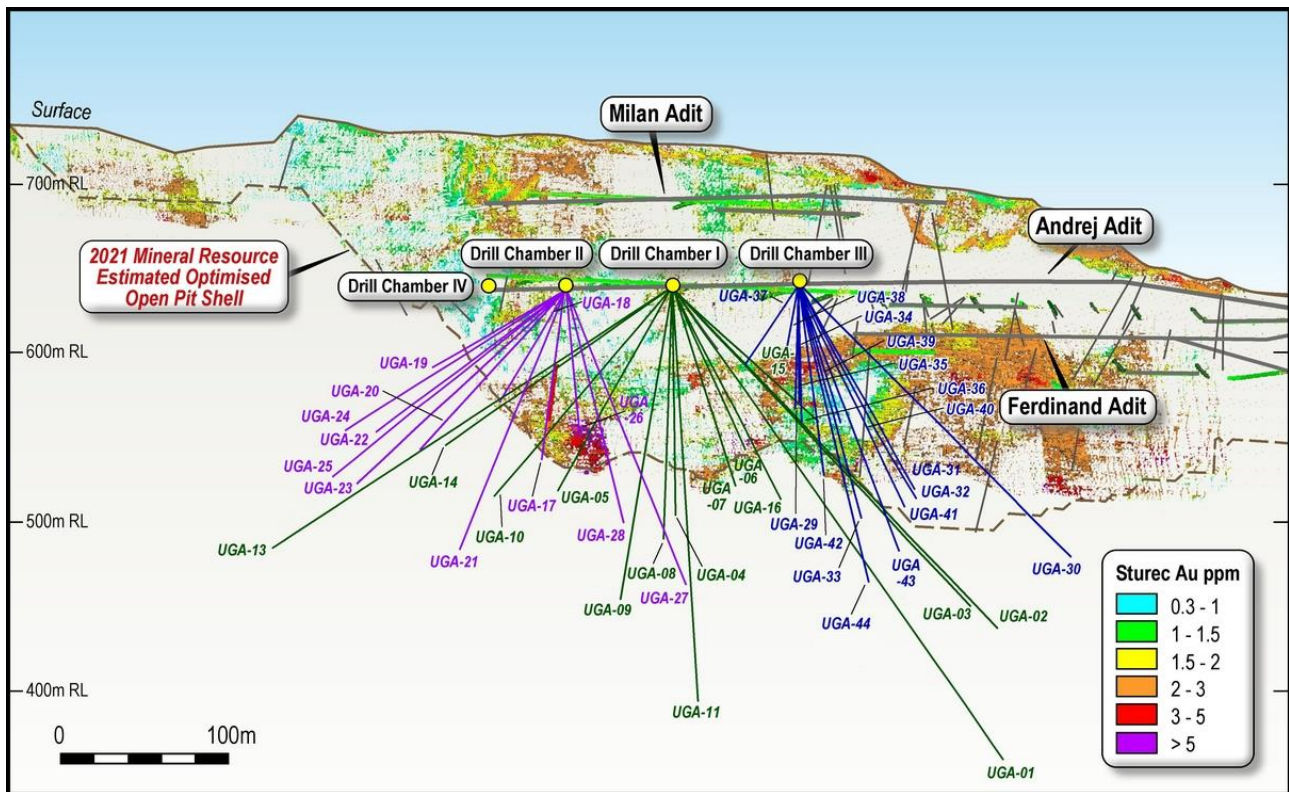
Figure 1: Long-section showing the traces of drill holes from the various drill chambers; shown relative to mineralisation within the existing Sturec Mineral Resource displayed as a 3D point cloud. This view is looking west
