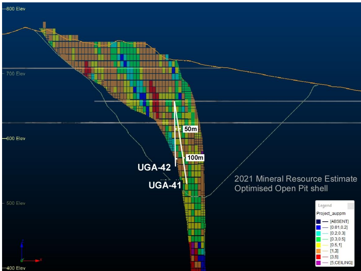
Figure 2: Cross-section through the existing Sturec Mineral Resource displayed as mineral resource blocks, which are 10m high and 5m. The path of UGA-42 is slightly into the page. This view is looking north.
