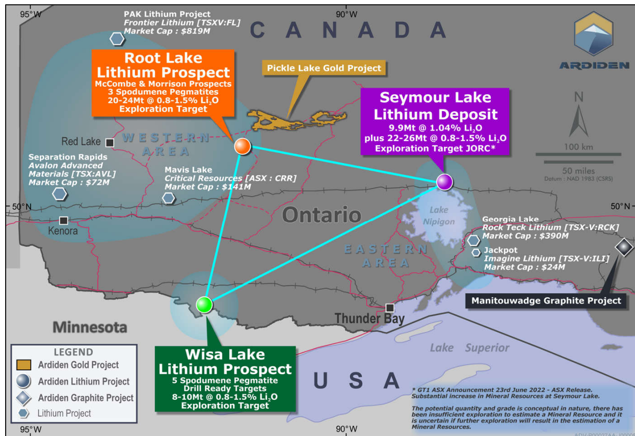
Figure 10- Location of Ardiden's Three Joint-Ventured Lithium Projects in NW Ontario
