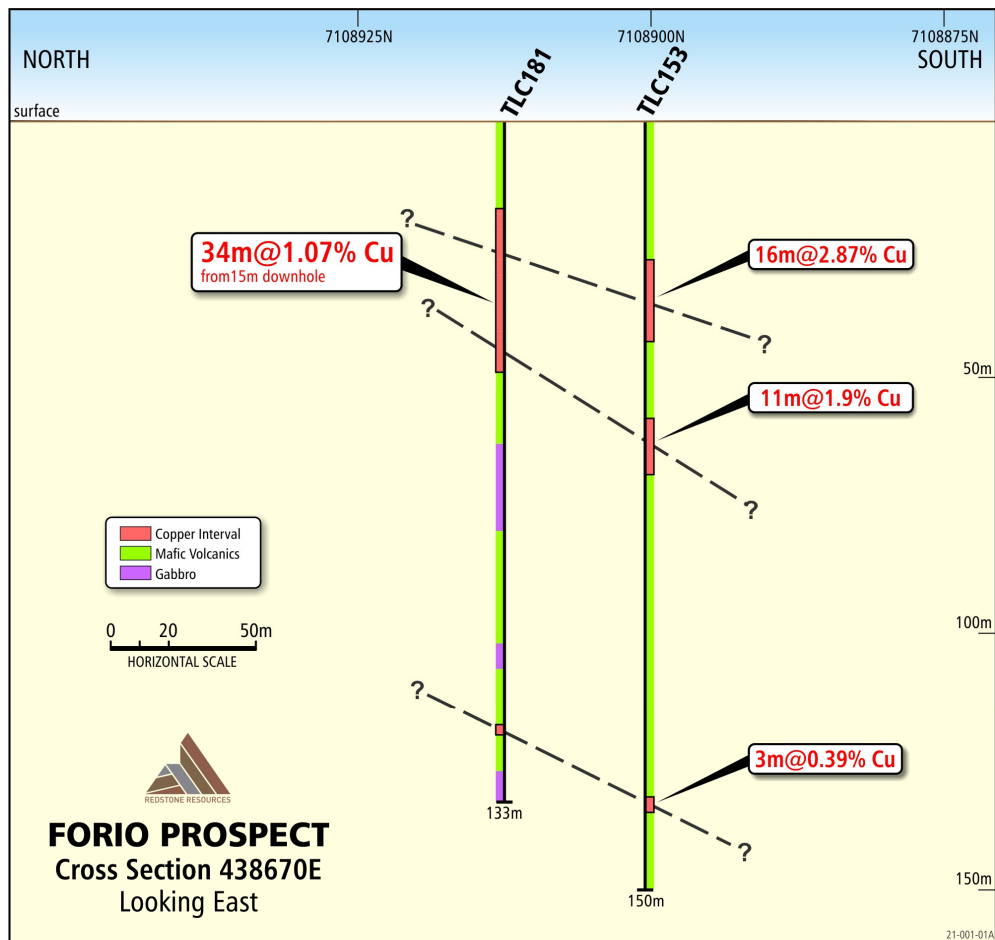
Figure 2 – Cross-section of RC drill hole TLC181 drilled at the end of 2021 at Forio to test for extension of the high grade mineralisation intersected in TLC153 in 2017. Cross-section is drawn along strike of the Forio vein system and looking towards the east. See text for further details.
