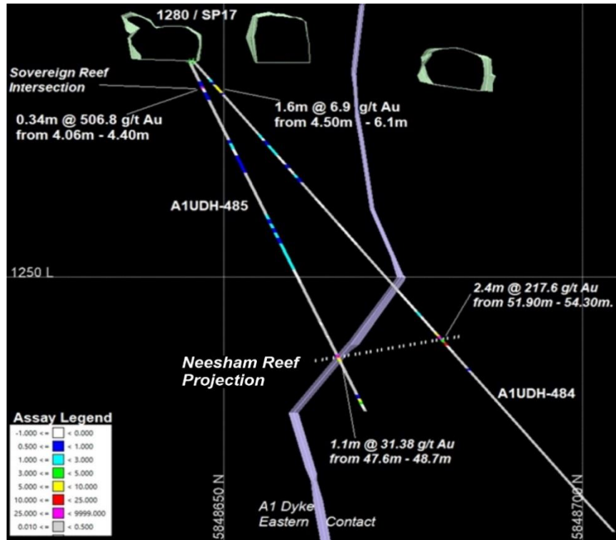
Figure 1: Long section looking west showing drilling traces, drives and the interpreted main dyke margin (purple)
