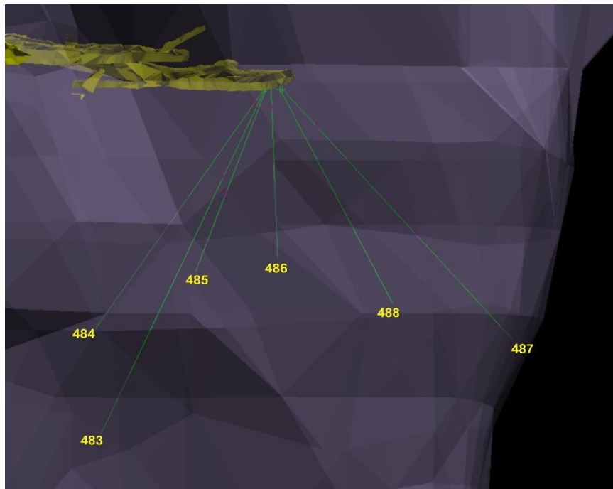
Figure 2: Long section looking east showing drilling traces, drive and the interpreted main dyke shape (purple)
