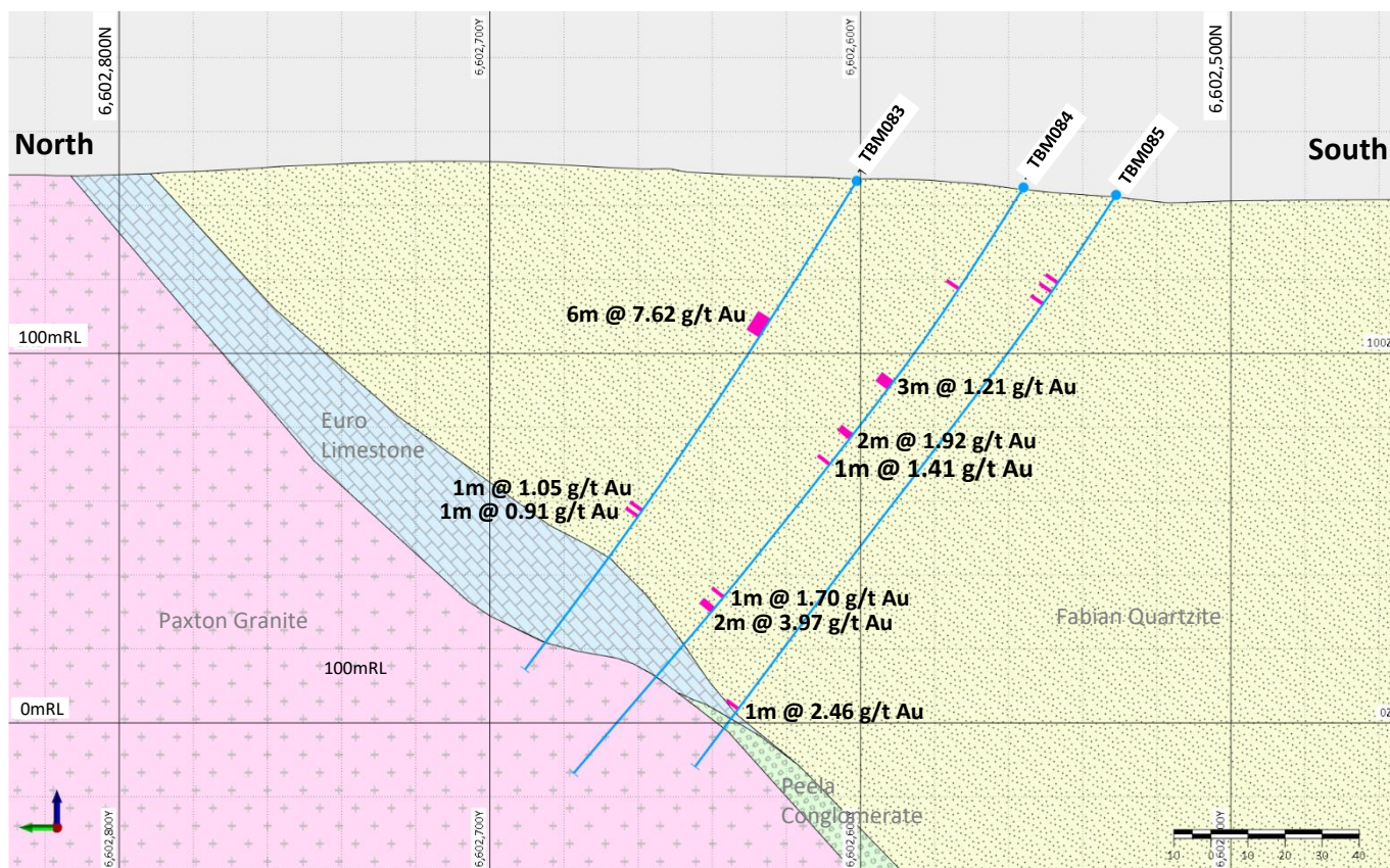
Figure 3 Cross Section A (454,580E)
