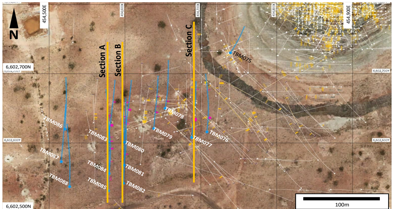
Figure 2 – Perseverance West drill hole location plan
