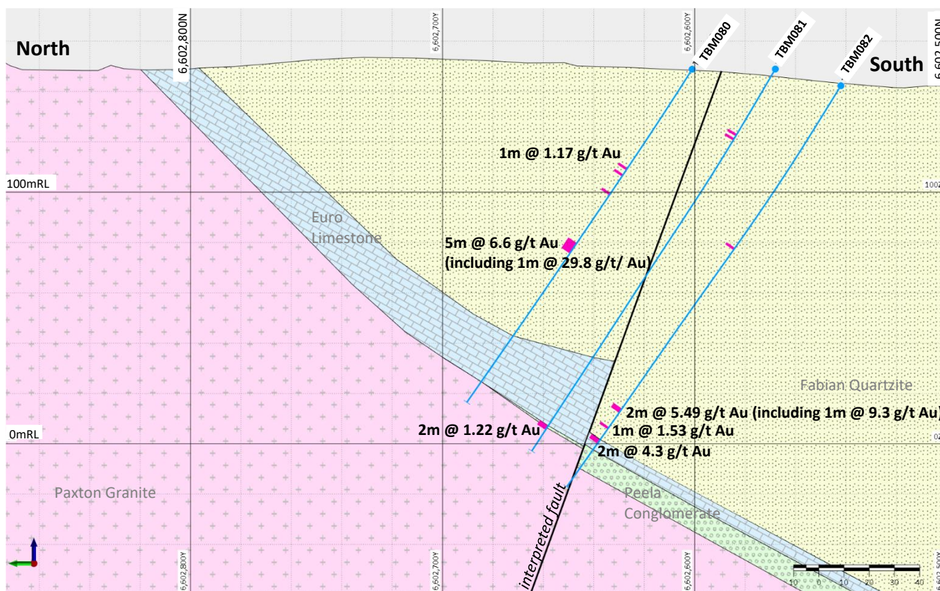
Figure 4 Cross section B (454,580E)
