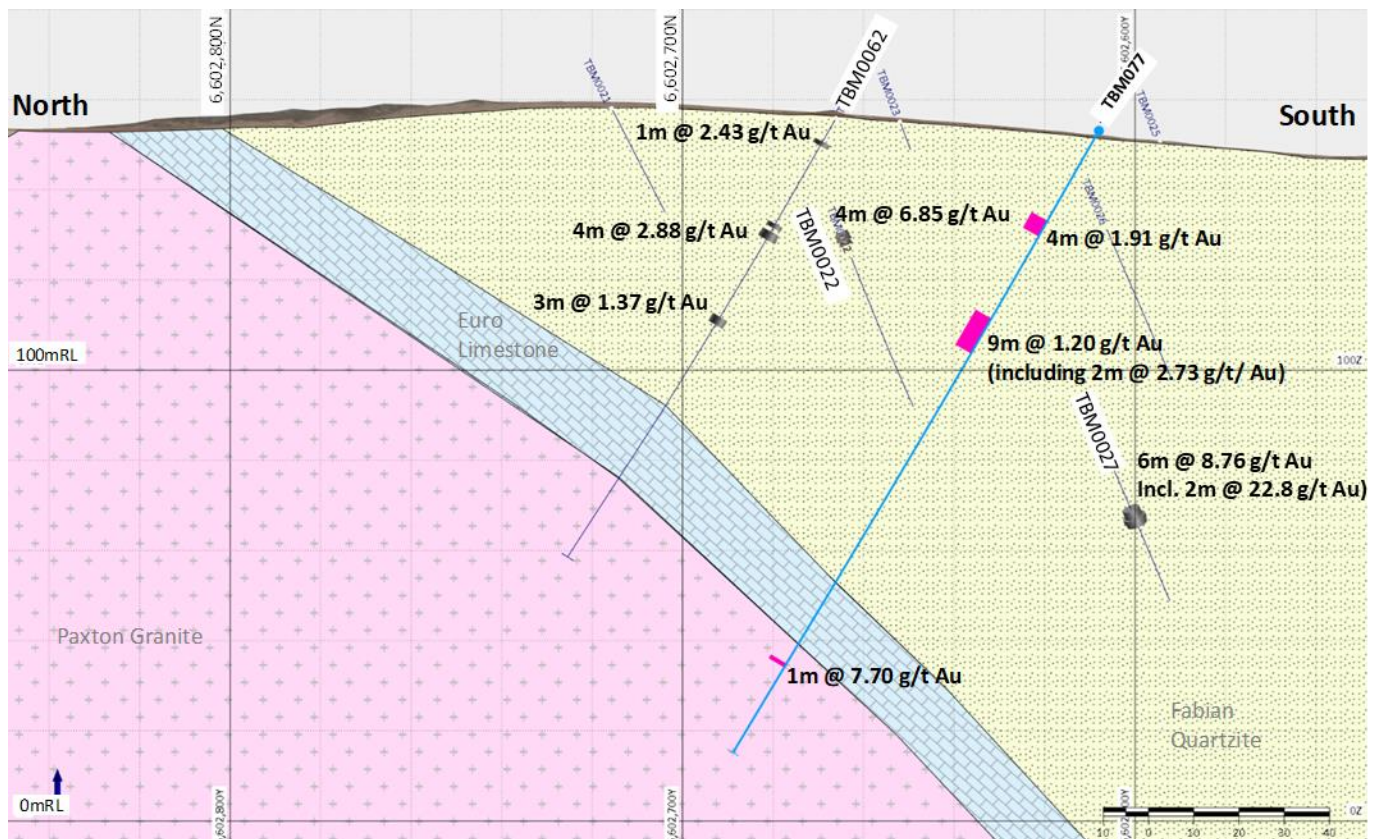
Figure 5 Cross section C (454,690E)
