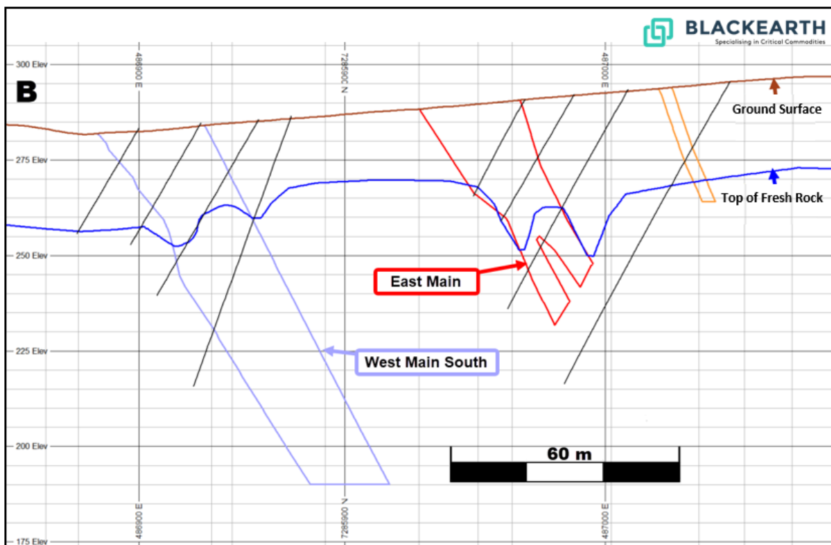
Figure 3 : Cross Section "B" depicting location of 2 main lenses (refer Figure 1)
