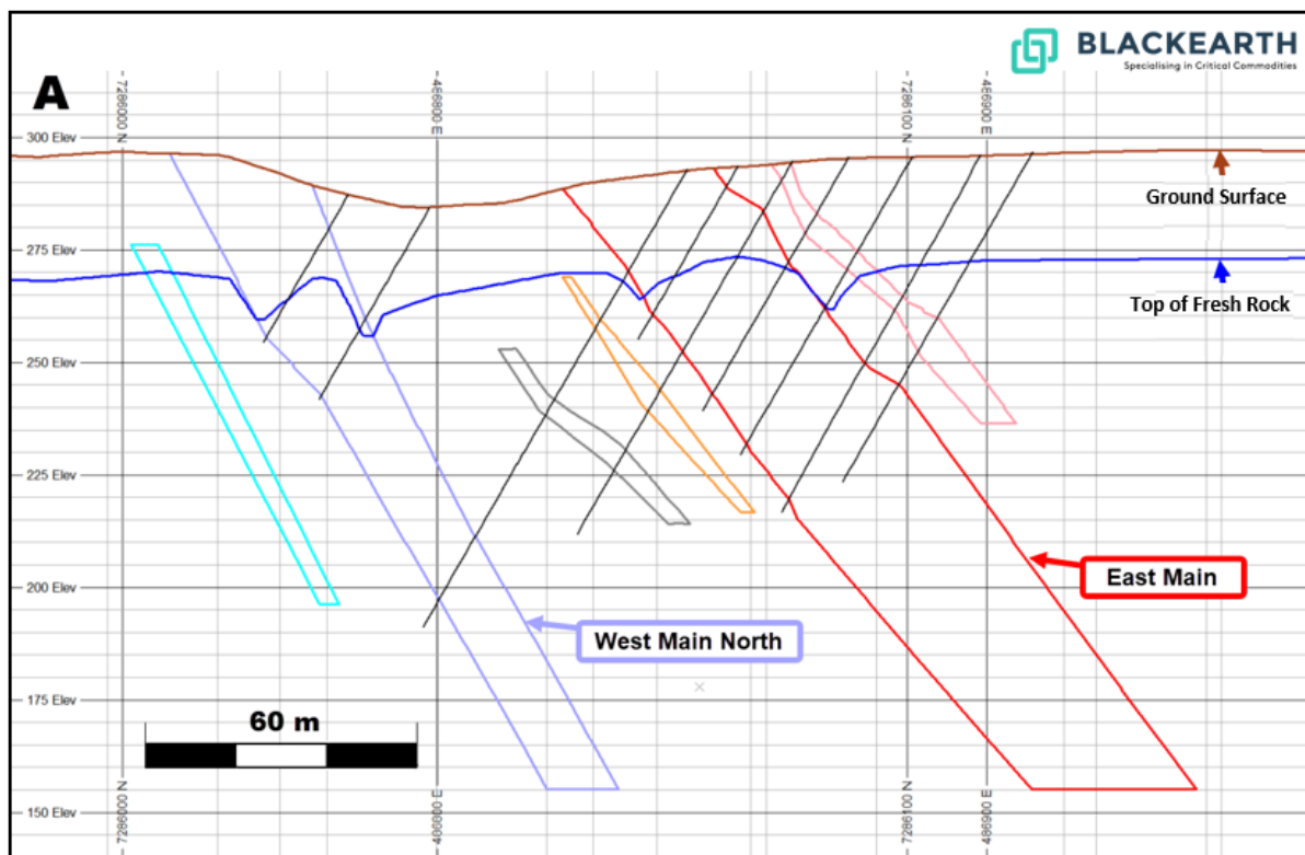
Figure 2 : Cross Section "A" depicting location of 2 main lenses (refer Figure 1)
