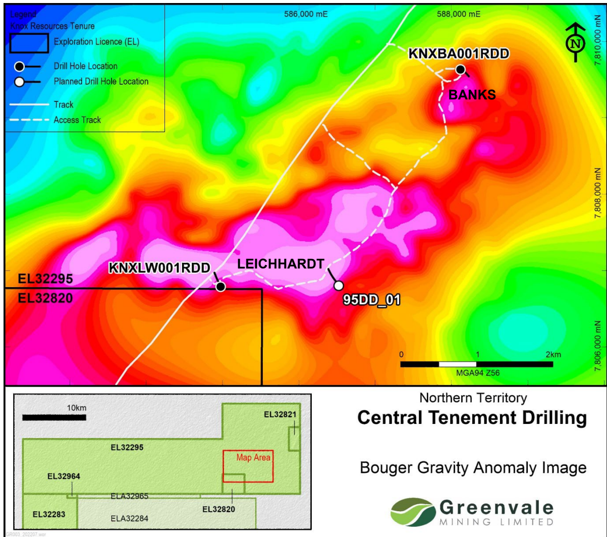
Figure 2: Gravity anomalies and location of planned and drilled holes.
