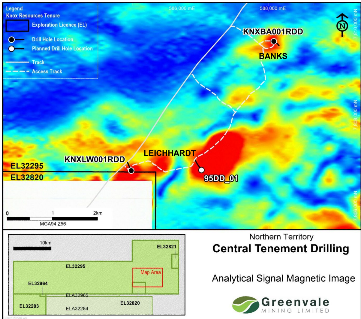
Figure 3: Magnetic anomalies and location of drilled and planned drill-holes.
