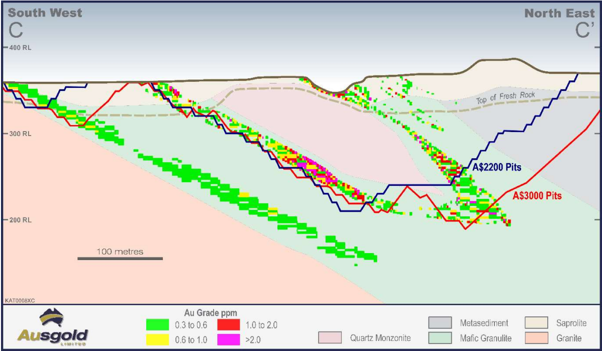
Figure 5: Jinkas cross-section C-C', looking north
