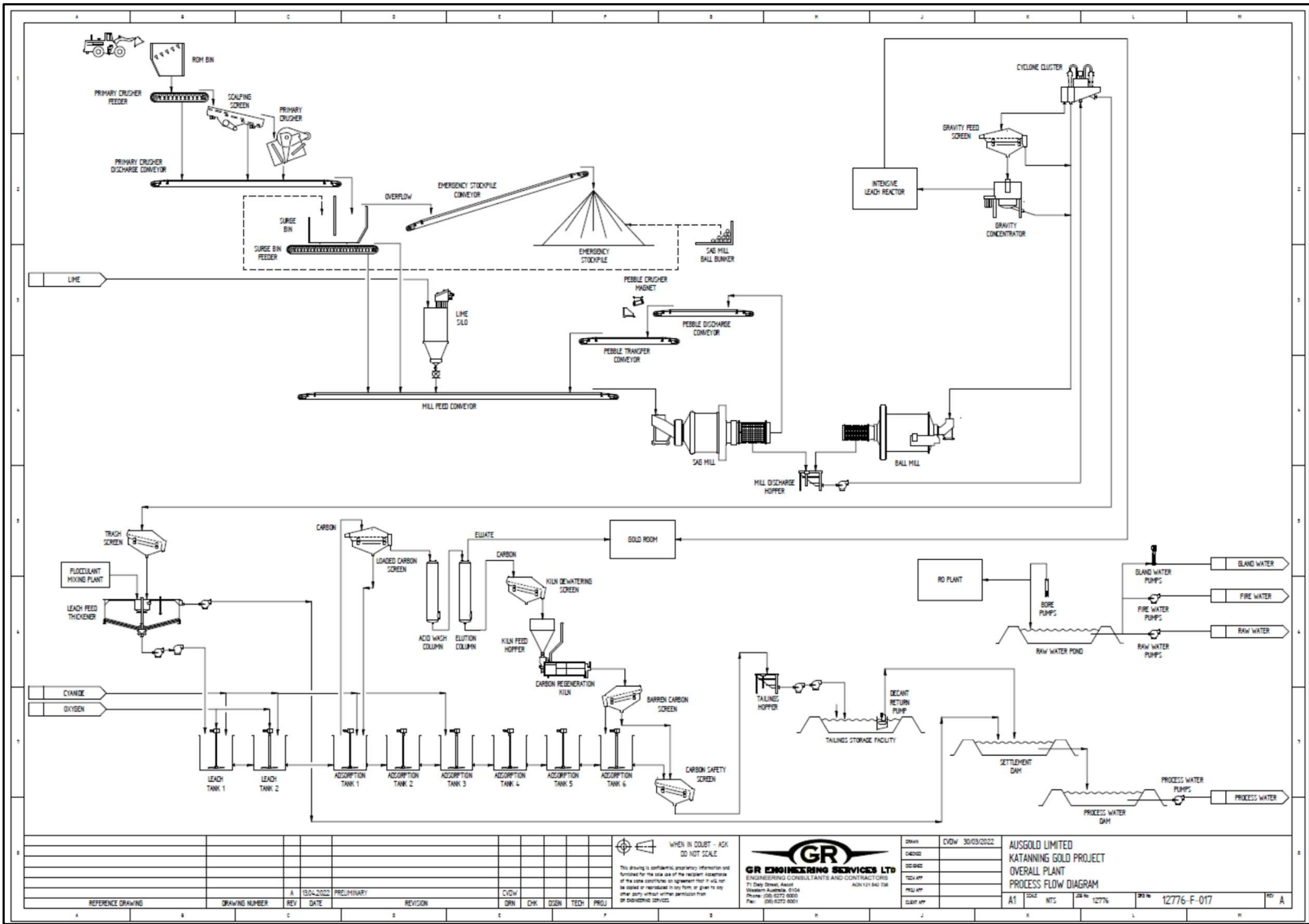
Figure 13: Process flowsheet
