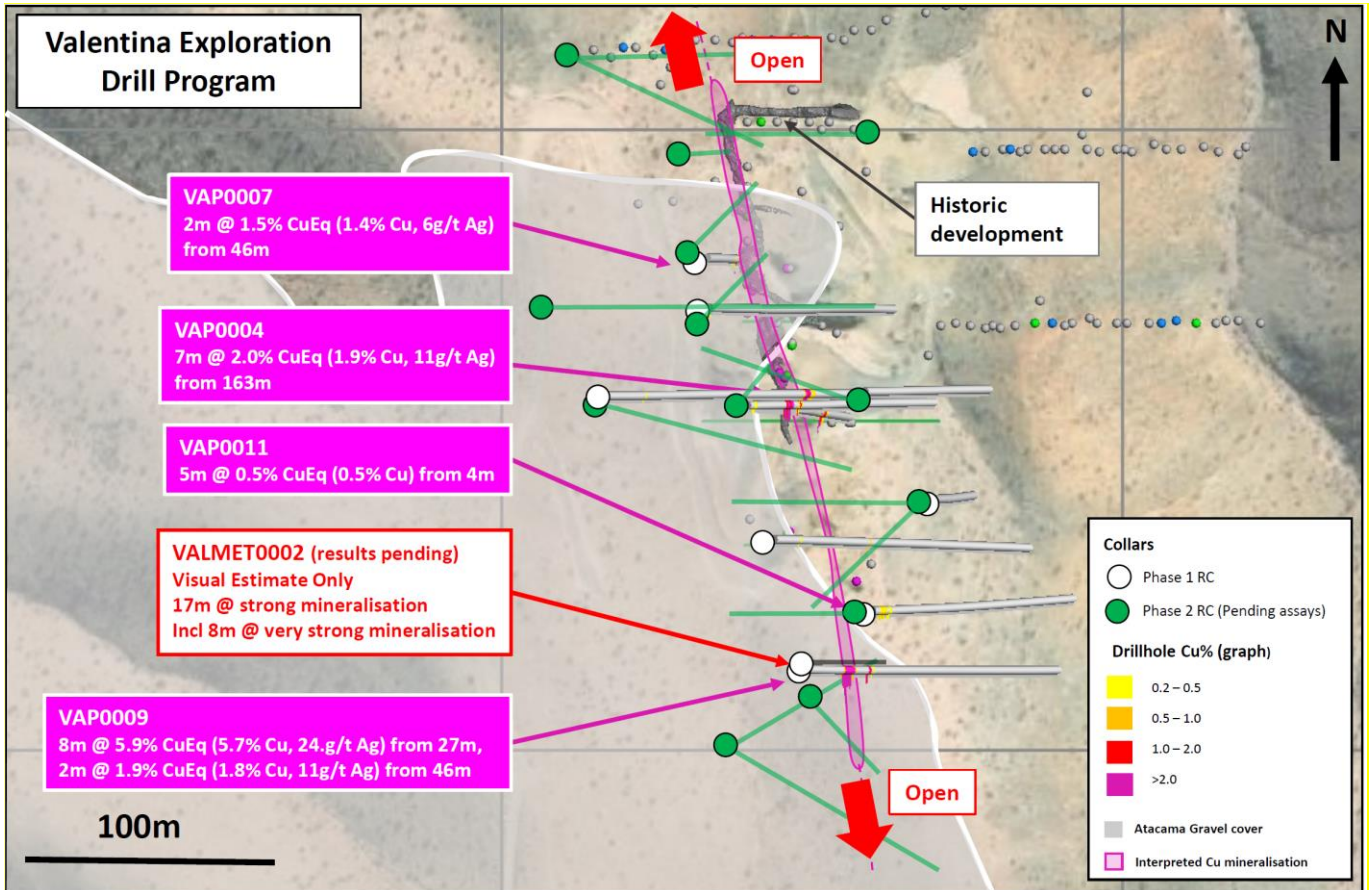
Figure 2. Location of drill holes in relation to the Valentina high grade copper deposit. Valentina is open along strike to the north and to the south underneath a 10 to 15m deep cover of gravel.
