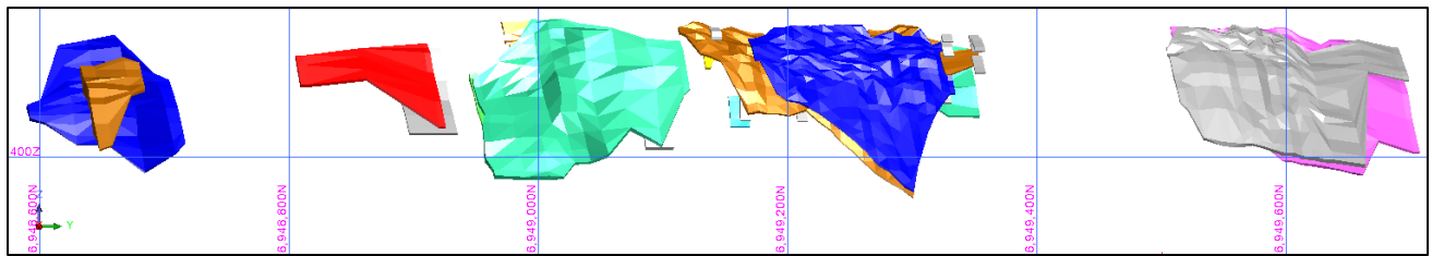
Figure 4 Long section view of wireframe interpretation for Challenger mineralisation looking WSW.
