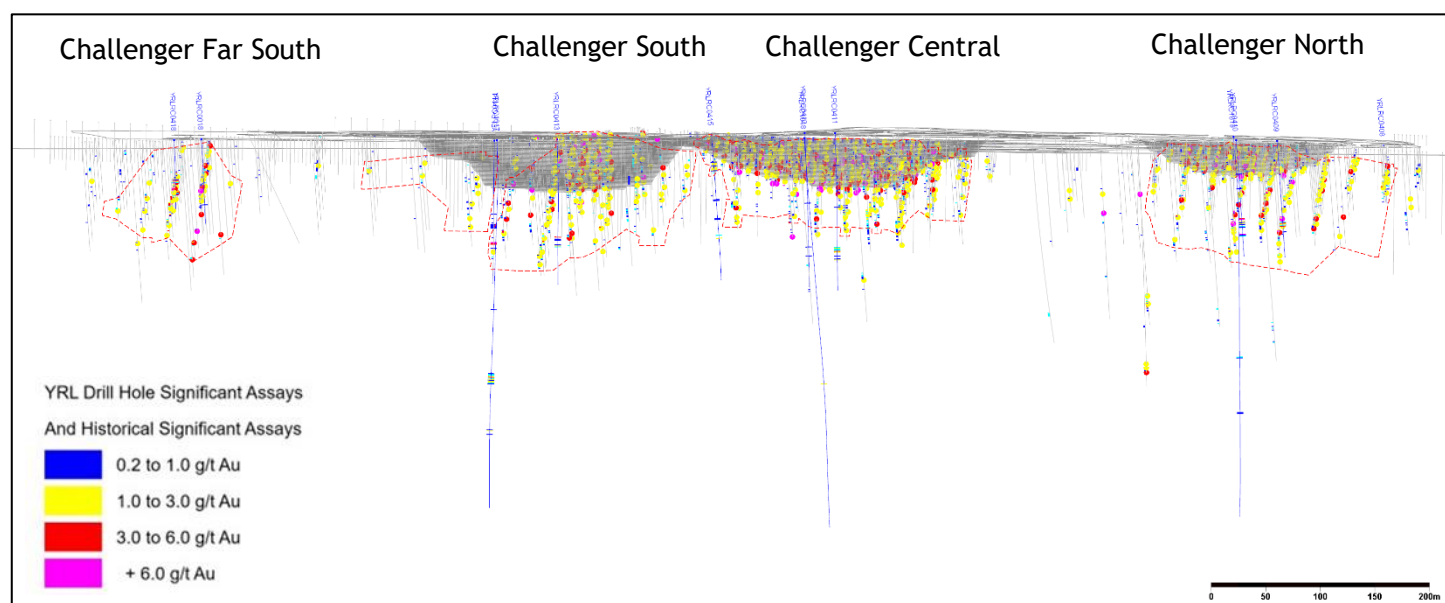
Figure 2 – Challenger Long Section looking WSW showing modelled wireframe outlines (red dash), historic pits (grey shading) historic (black) and Yandal (blue) drill traces and significant intercepts
