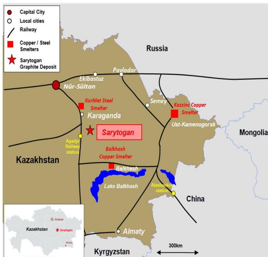
Figure 2 - Sarytogan Graphite Deposit location
