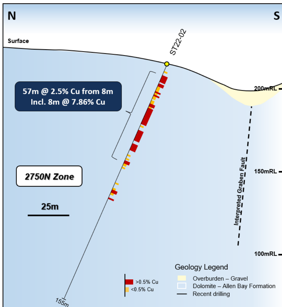
Figure 2: Schematic geological section at 466200E showing drilling and mineralised intervals.
