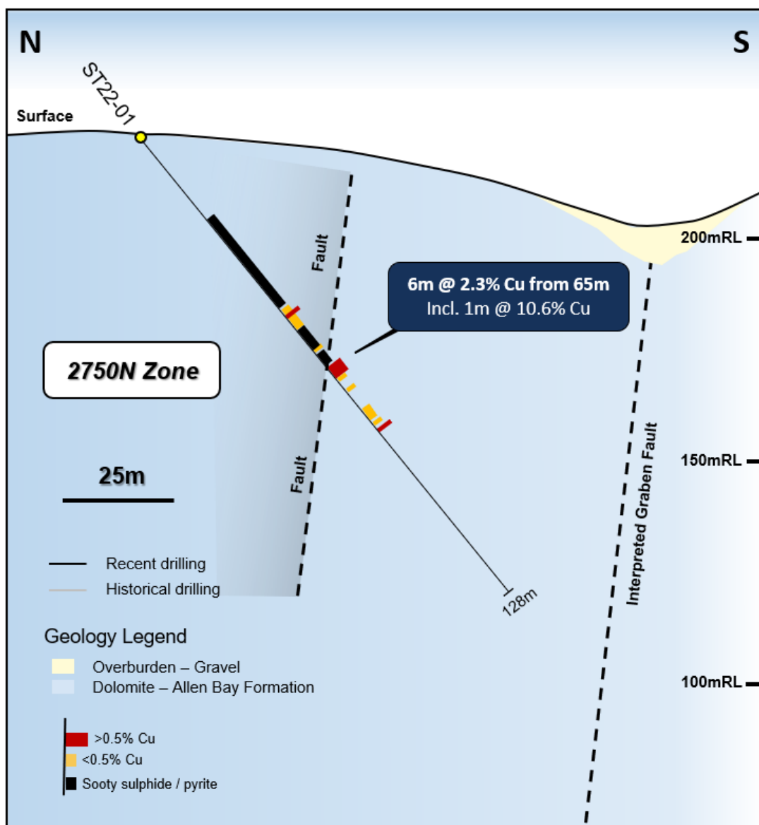
Figure 4: Schematic geological section at 466230E showing drilling and mineralised intervals.
