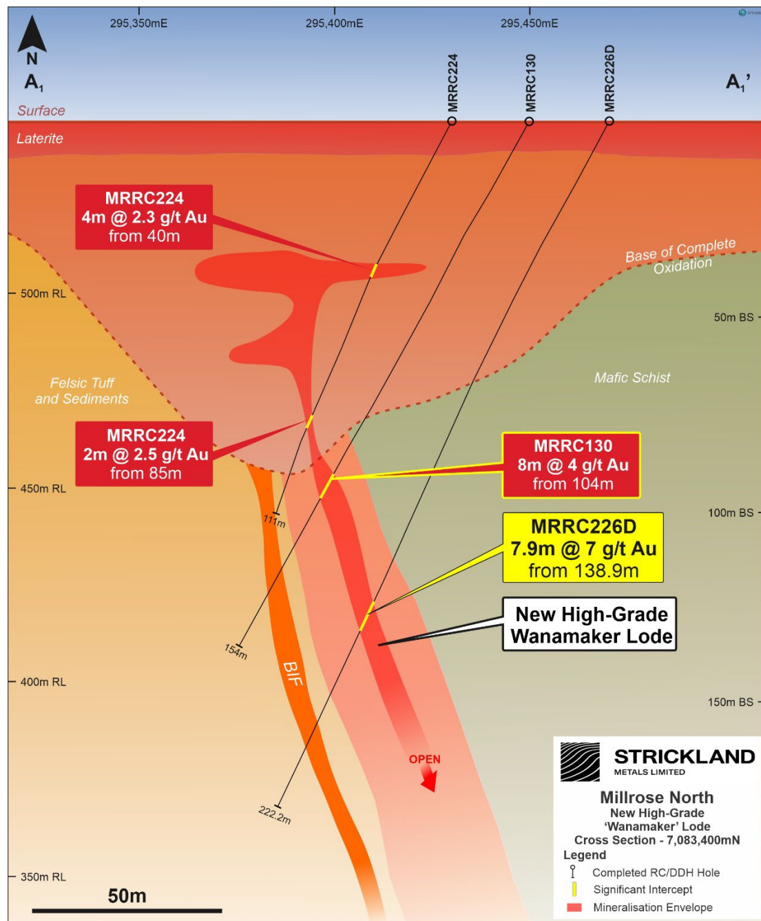
Figure 1: Wanamaker Cross Section
