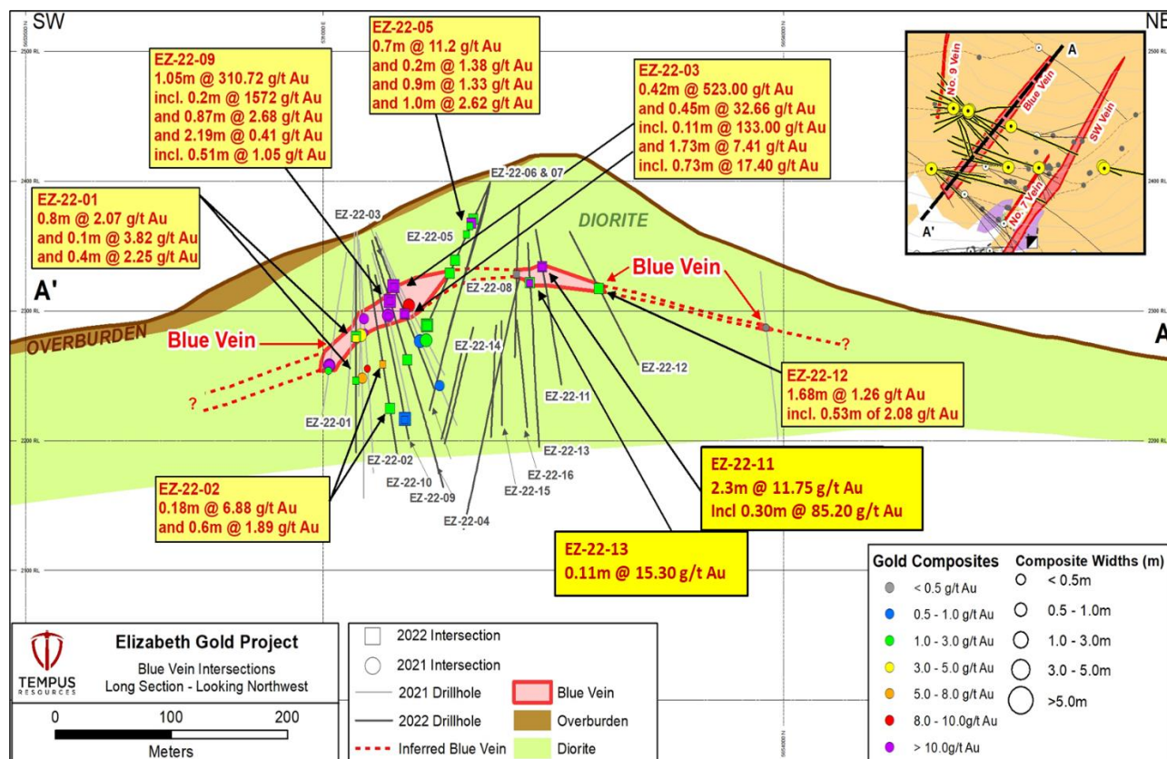
Figure 2 – Elizabeth Blue Vein long section (looking northwest)
