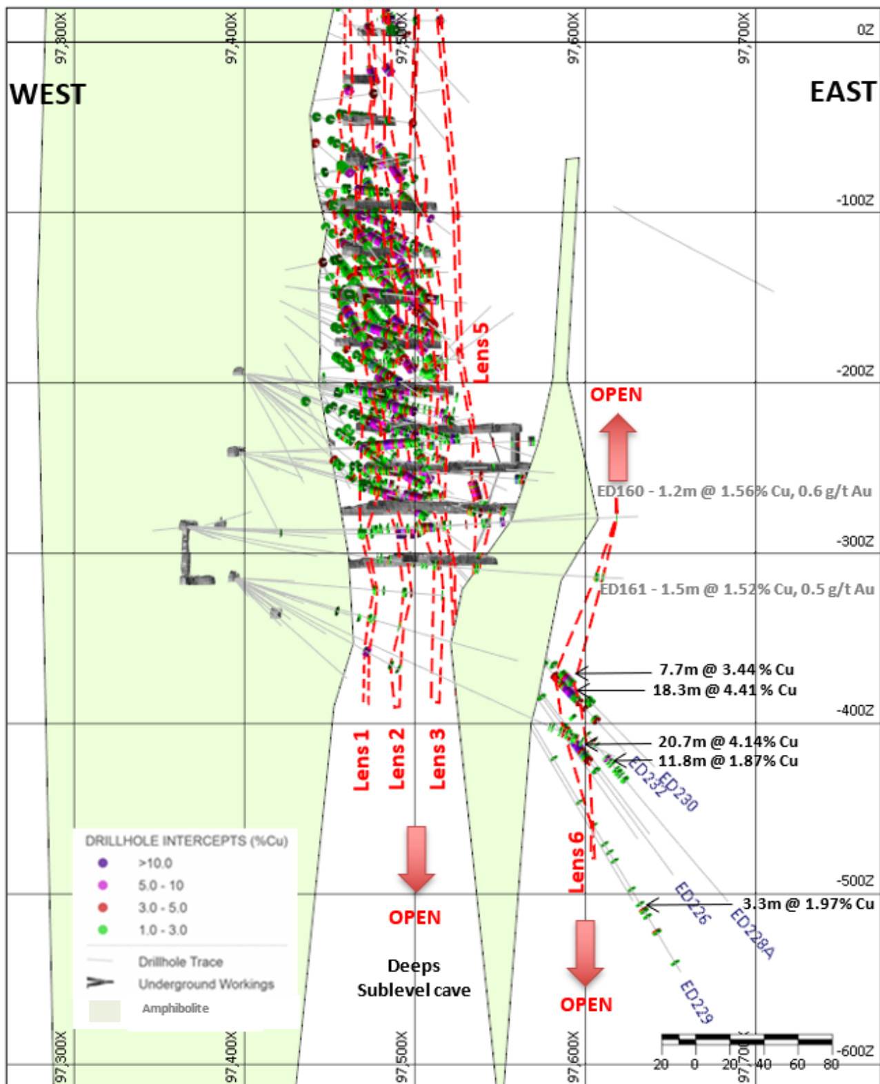
Figure 1. Cross section of Deeps drilling and Lens 6 (looking north). Drillhole intercepts are reported as estimated true widths.
