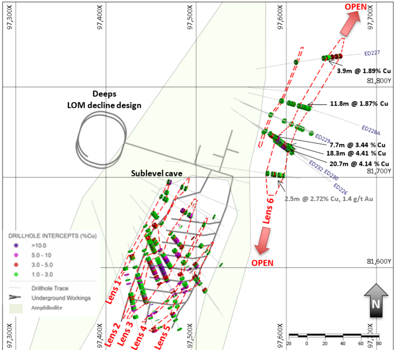
Figure 2. Plan view of Deeps drilling and Lens 6. Drillhole intercepts are reported as estimated true widths.
