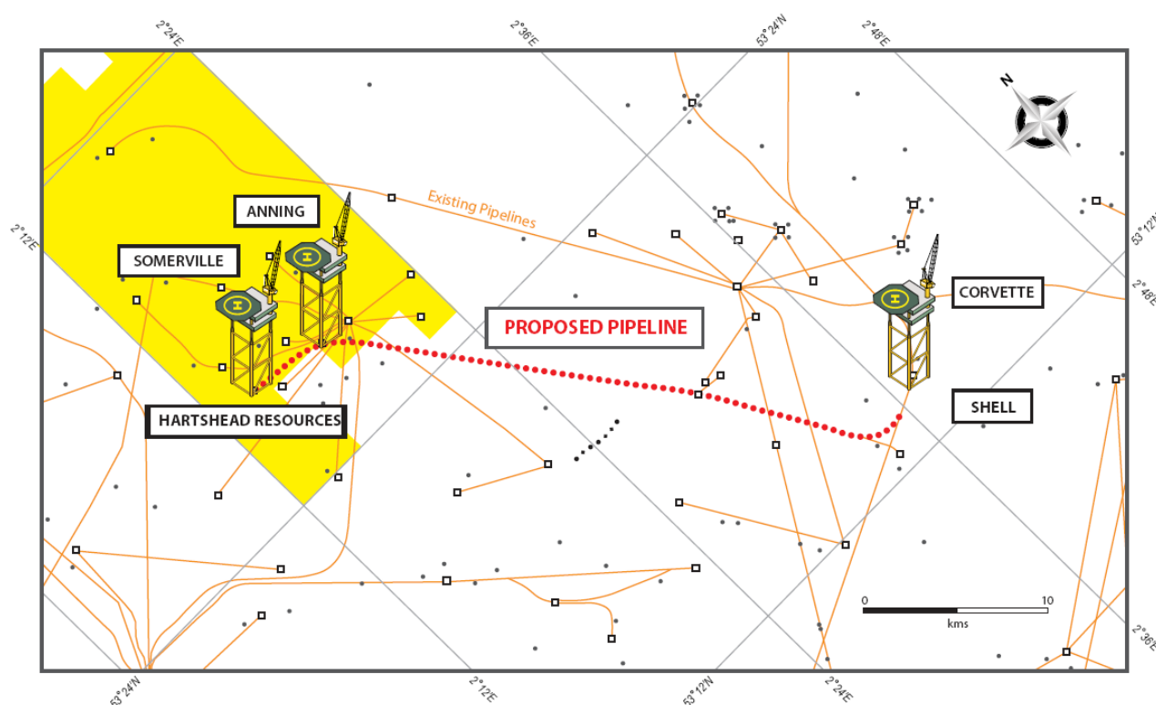
Figure 18. Preferred tie-in point of Anning and Somerville fields to Shell's infrastructure (Corvette and Leman-A platforms)
