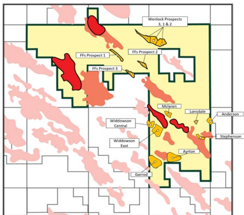
Figure 10. Phase III exploration portfolio prospects and leads map.
