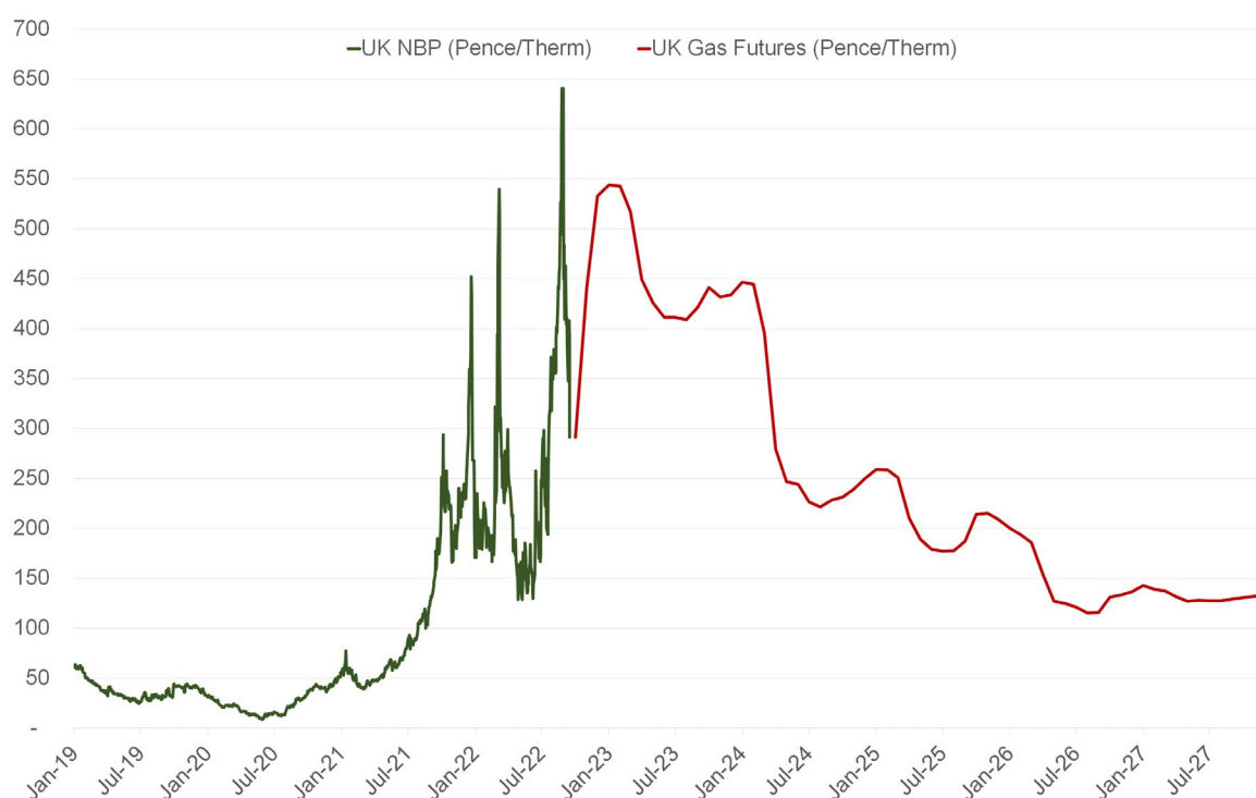
Figure 12. UK NBP historical and future pricing (Dated: 16 September 2022)
