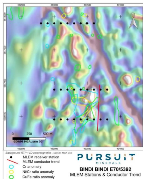
Figure 9: Bindi Bindi MLEM plate relative to geochemical anomalism
