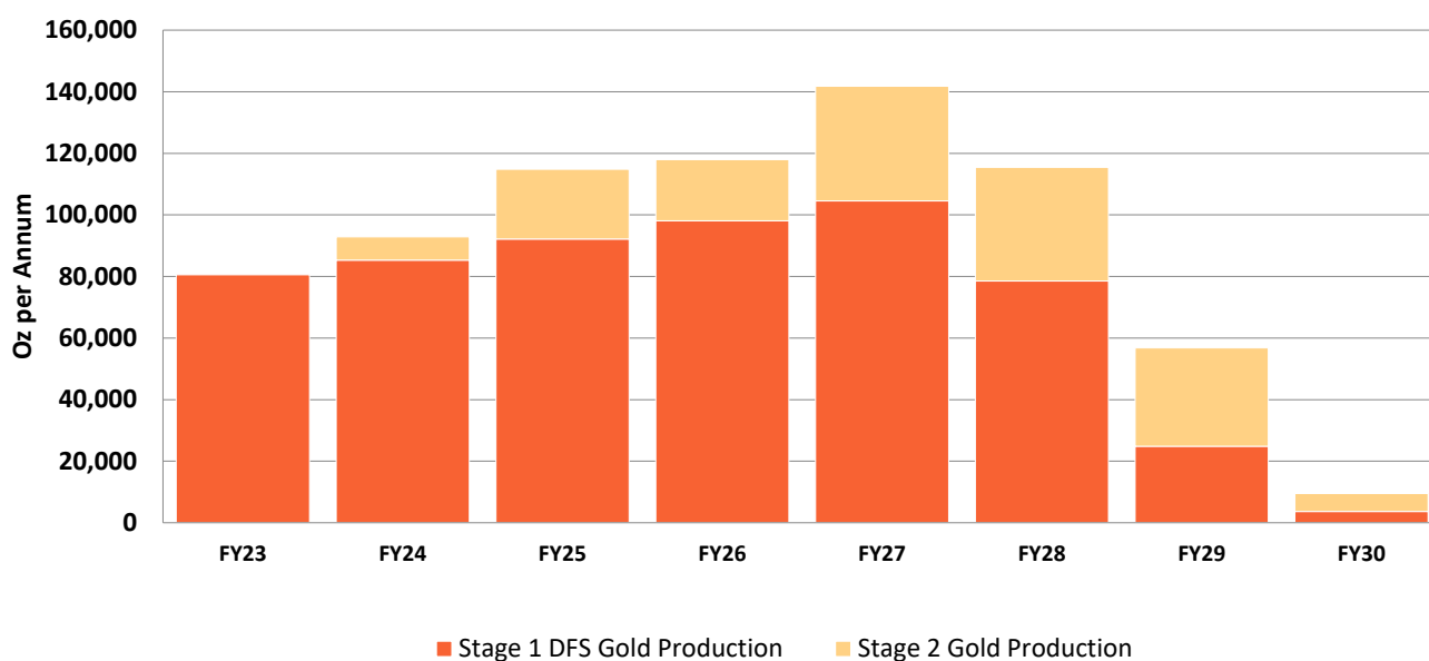
Figure 5: Annualised production profile for combined Warrawoona DFS production (Stage 1) with the Sulphide Plant (Stage 2)
