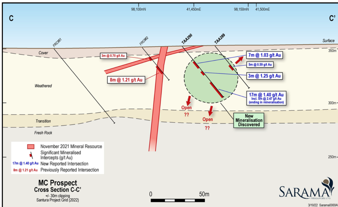
Figure 5 – Cross Section C-C' (Looking NNE)
