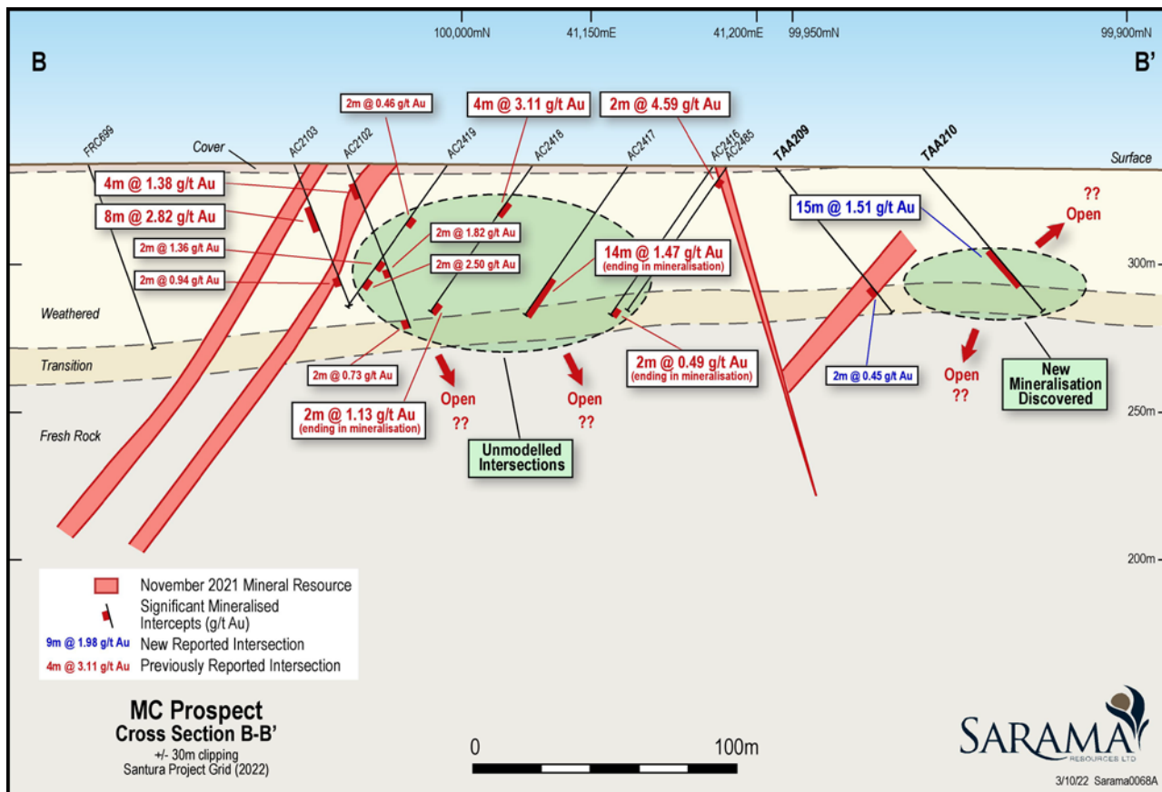
Figure 4 – Cross Section B-B' (Looking NNE)
