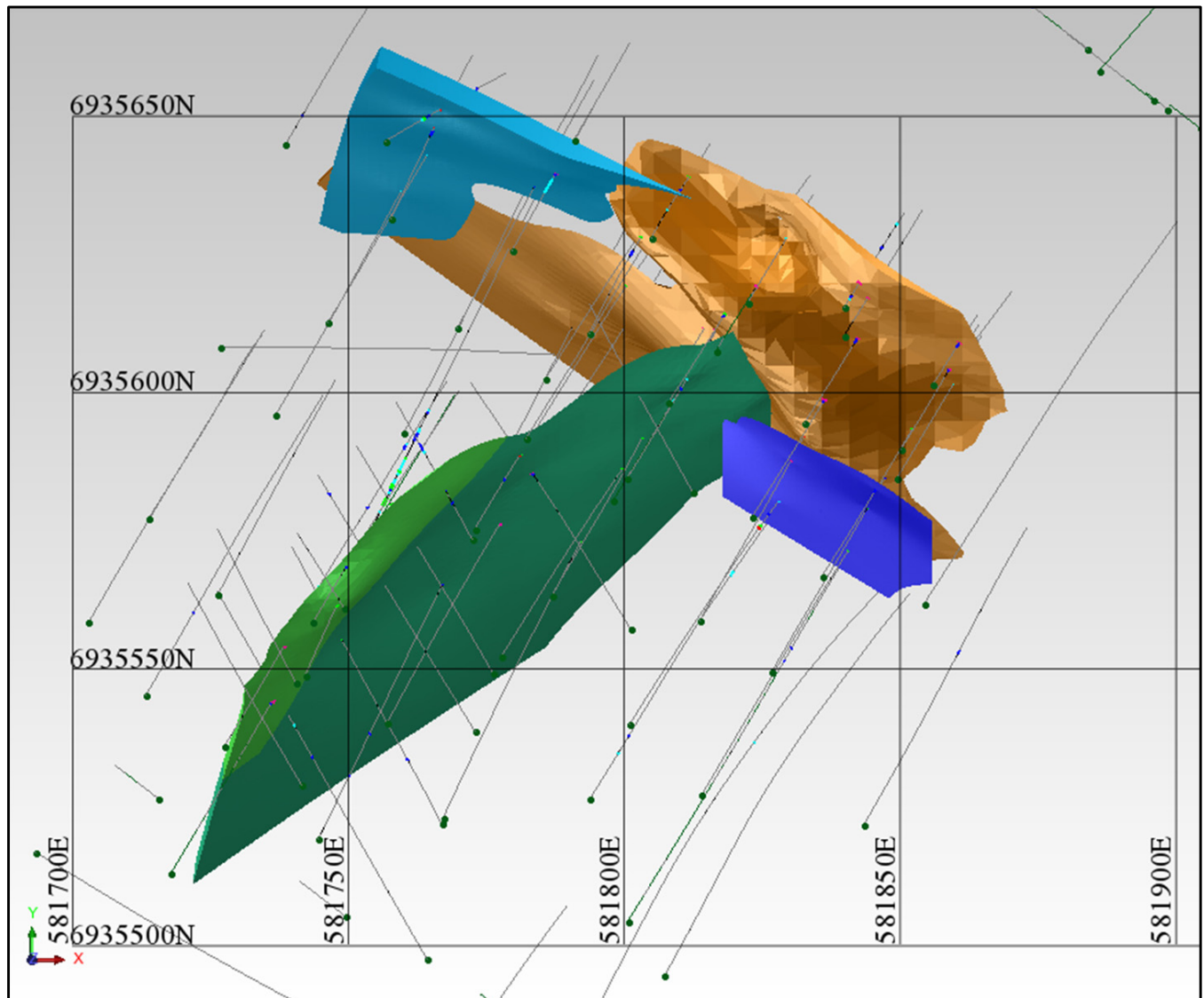
Figure 5: Schematic 3D model showing White Heat and Mosaic lodes along the High-grade Break of Day trend, Cue Project (Brown and blue lodes – White Heat, Green lode – Mosaic)
