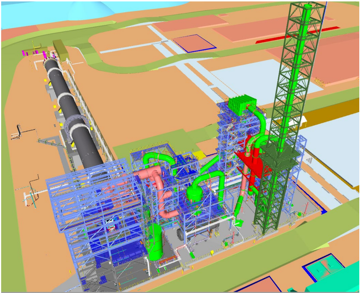
Figure 1: 3D Render of Feed Hood Building and Stack Support Tower to be erected
