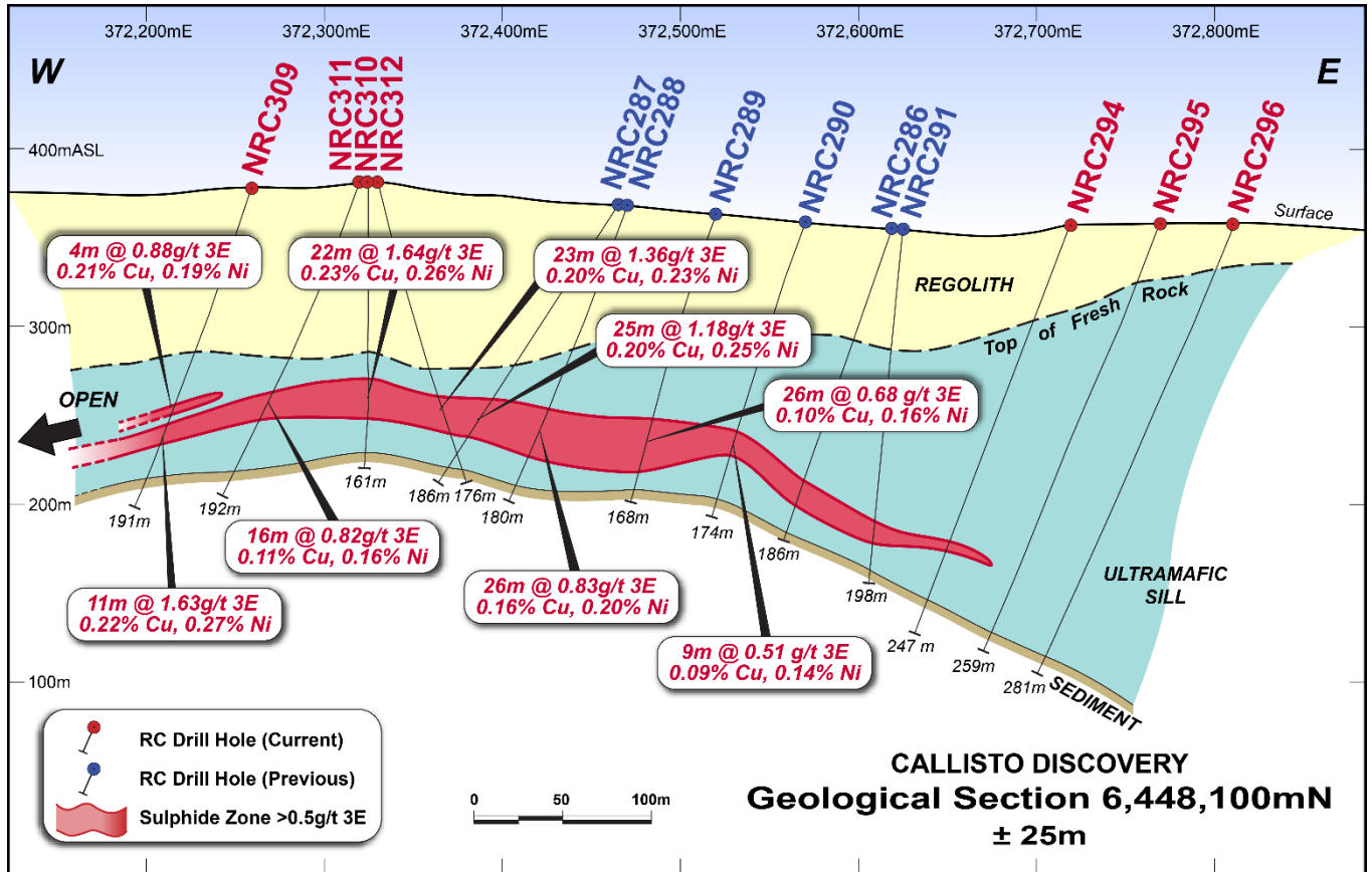
Figure 2 — Callisto geological interpretation section 6,448,100. Mineralisation is continuing to the west where grade appears to be increasing (NRC309 compared with drill hole NRC311 on left hand side of section).
