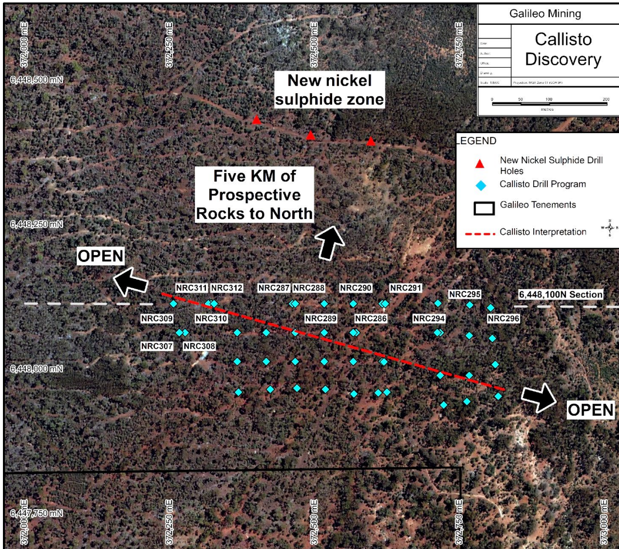
Figure 3 — Plan map of drilling with 6,448,100N section line (Figure 2). Newly identified nickel sulphide zone is shown (ASX Announcement dated 10/10/2022) with an additional five kilometres of prospective rocks to the north. Interpretation of the metal distribution plunge within the sulphide zone at Callisto is shown by the red dotted line, open in both directions. Diamond drilling is ongoing at Callisto while the RC drill rig continues to test targets to the north.
