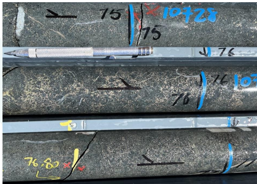
Figure 1: 22B1DD002 (included in the 76.8-85.4 metre interval – NQ core 47.6mm diameter). Strongly mineralised pyroxenite with fine-grained pyrrhotite and chalcopyrite with lesser pyrite, including a band of massive chalcopyrite and oxidised pyrrhotite between 84.0-.84.1m, Within a 20.7 metre zone of sulphide mineralisation. 1 Mineralisation is mottled and massive.
