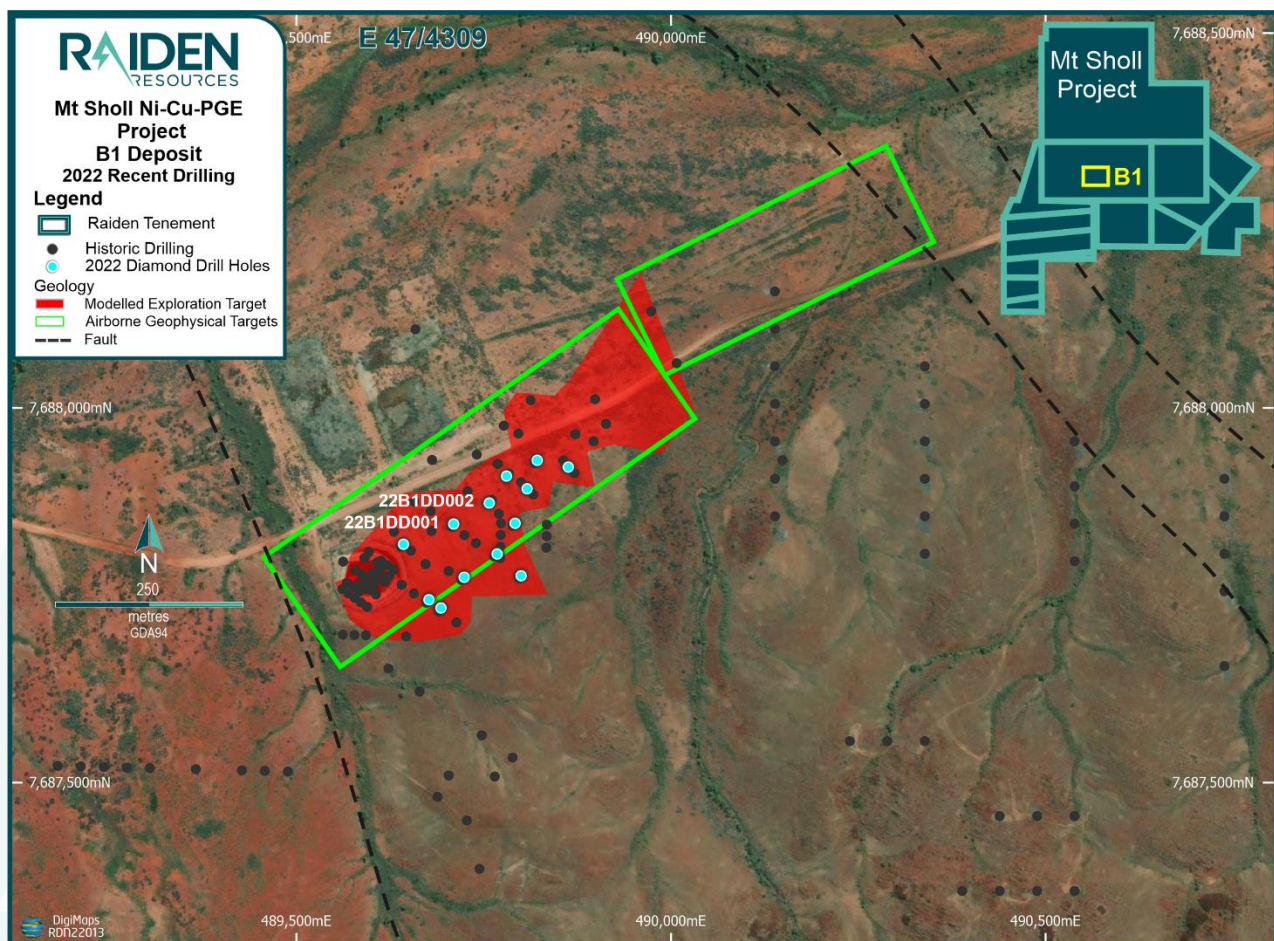
Figure 4: Mt Sholl B1 Deposit area with 2022 planned/drilled (blue dots), historic hole locations (black dots) over interpreted geology and JORC Exploration target 3 (red). The deposit remains open along strike and depth.
