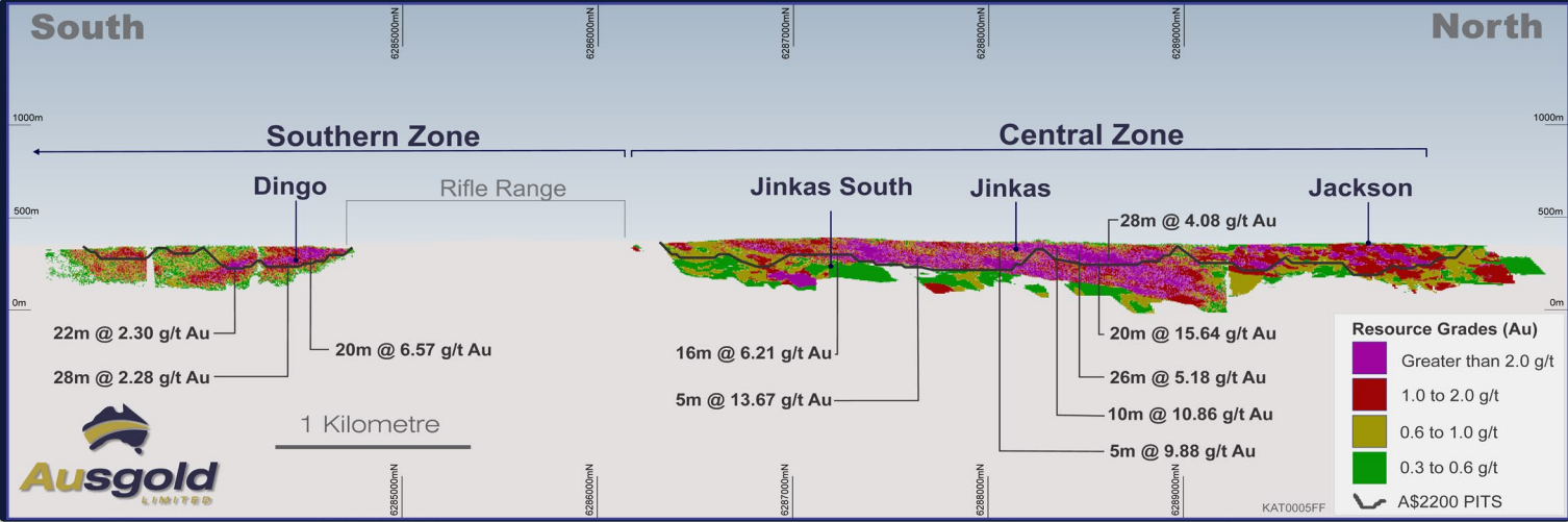
Katanning Long section through KGP
