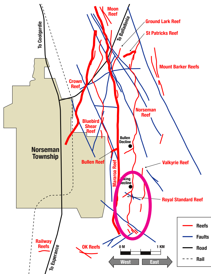
Schematic View of Mainfield Reefs
