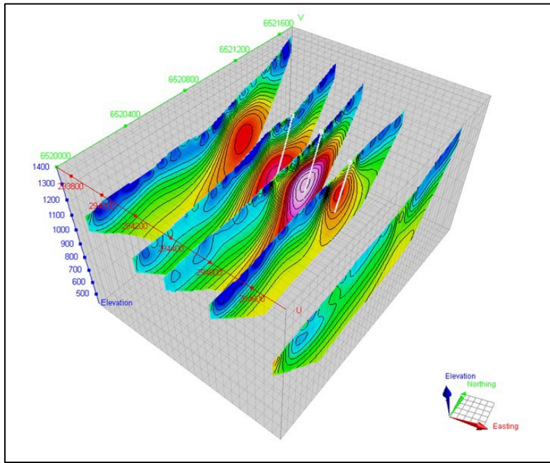
3D view from above and looking north on PDIP chargeability inversion model cross sections at the Anico prospect and proposed drillhole locations.(ASX announcement, 10 October2022)
