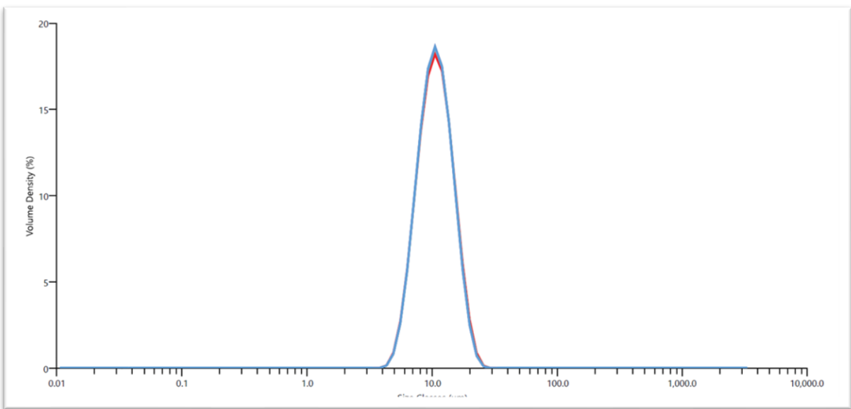
Figure 5: Size distribution of the spheroidised product
