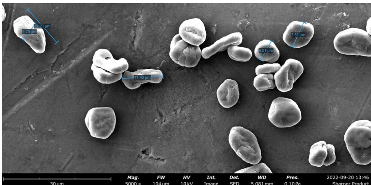
Figure 1: Spheroidised graphite particles under the electron microscope
