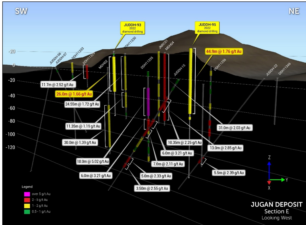
Figure 5: Cut-away section of the main Jugan mineralised body showing the location of JUDDH 95, which has extended an area of higher-grade mineralisation further to the NE from historic holes JNRC01 and MDH04 towards DDH 1336.
