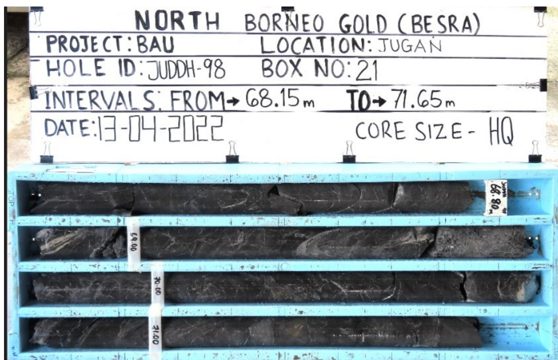
Figure 6: Core recovered from JUDDH-98 from portion of the 13m interval 61m-74m assaying at 4.33 g/t Au, containing interval 65m-71m @ 7.12g/t Au and 70m-71m @13.5 g/t Au.
