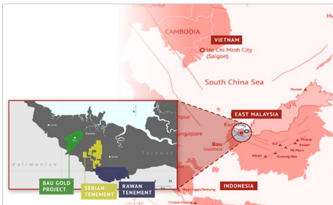
Figure 8: Location of Bau Gold Project. Inset shows tenement interests within Sarawak.
