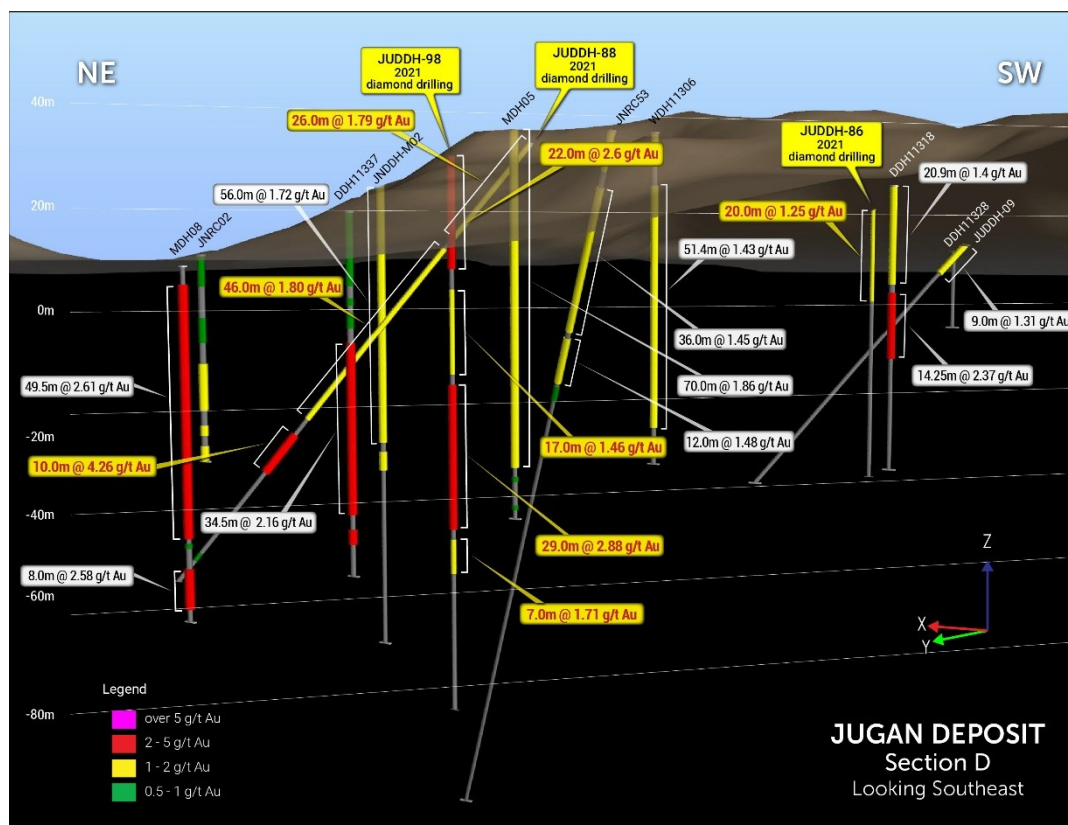
Figure 4: Cut-away section of the main Jugan mineralised body showing the locations of JUDDH 98, which has extended an area of higher-grade mineralisation across portion of the main body of Jugan mineralisation.
