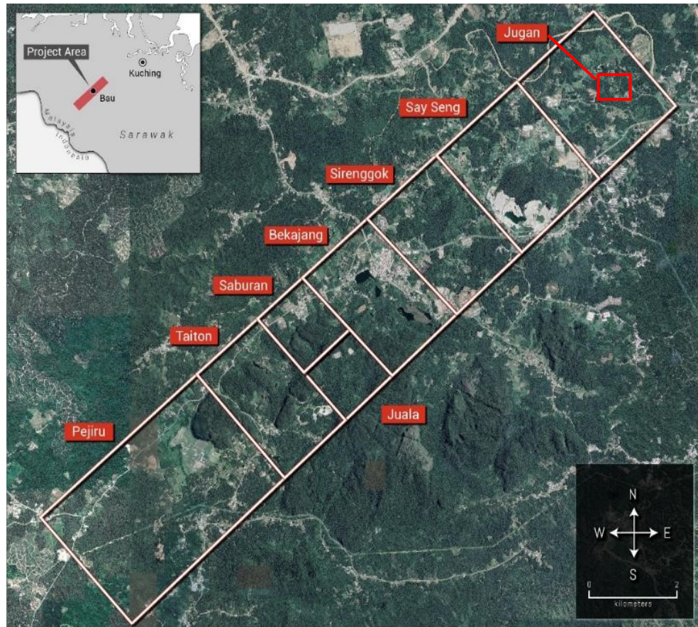
Figure 7: Location of the Jugan Sector (highlighted within red box) at the far northeast of the Bau Gold Field corridor, approximately 25 km from Sarawak's capital, Kuching (inset).
