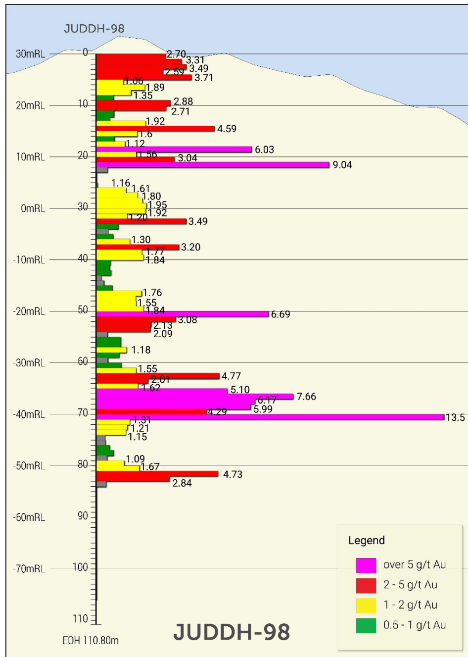
Figure 2: JUDDH-98, showing intercepted mineralisation grades based on nominal, true, 1m sample widths. JUDDH-98 intercepted significant intervals of higher than average historical global grades (1.5-1.6 g/t Au) including a maximum of 13.5 g/t Au.
