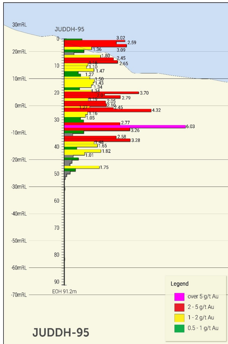
Figure 3: JUDDH-95, showing intercepted mineralisation grades based on nominal, true, 1m sample widths. Virtually continuous mineralisation extends from the surface down to 45m near the interpreted footwall thrust, including an interval with a maximum grade of 6.03 g/t Au.
