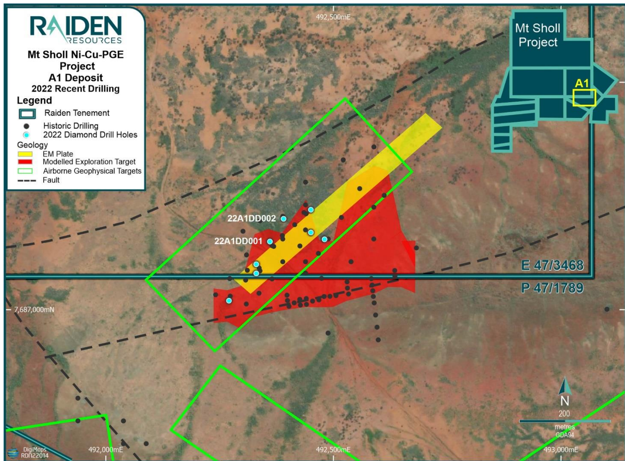
Figure 6: Mt Sholl A1 Deposit area with 2022 planned/drilled (blue dots) & historic hole locations over interpreted geology and JORC Exploration target 3 (red)
