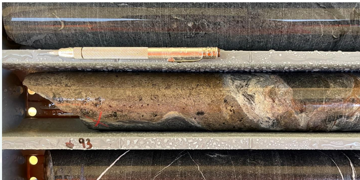
Figure 2: 22B1DD004 (92.2-92.4 metre interval – NQ core 47.6mm diameter). Strongly mineralised pyroxenite with fine-grained semi-massive pyrrhotite mineralisation, with lesser chalcopyrite and pentlandite, within a 32.8 metre zone of sulphide mineralisation. 1
