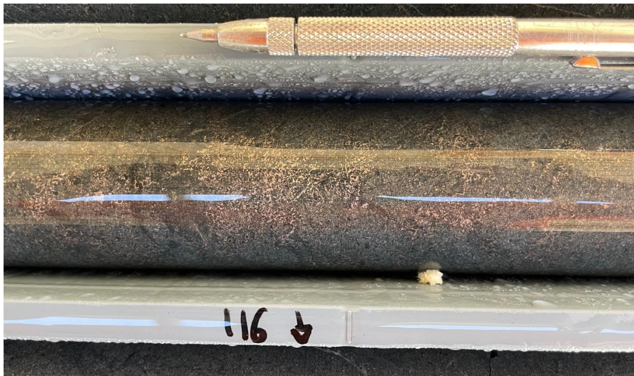
Figure 3: 22B1DD004 (approx. 115-116 metre interval – NQ core 47.6mm diameter). Strongly mineralised pyroxenite with fine-grained disseminated pyrrhotite mineralisation, with lesser chalcopyrite and pentlandite, within a 32.8 metre zone of sulphide mineralisation. 1
