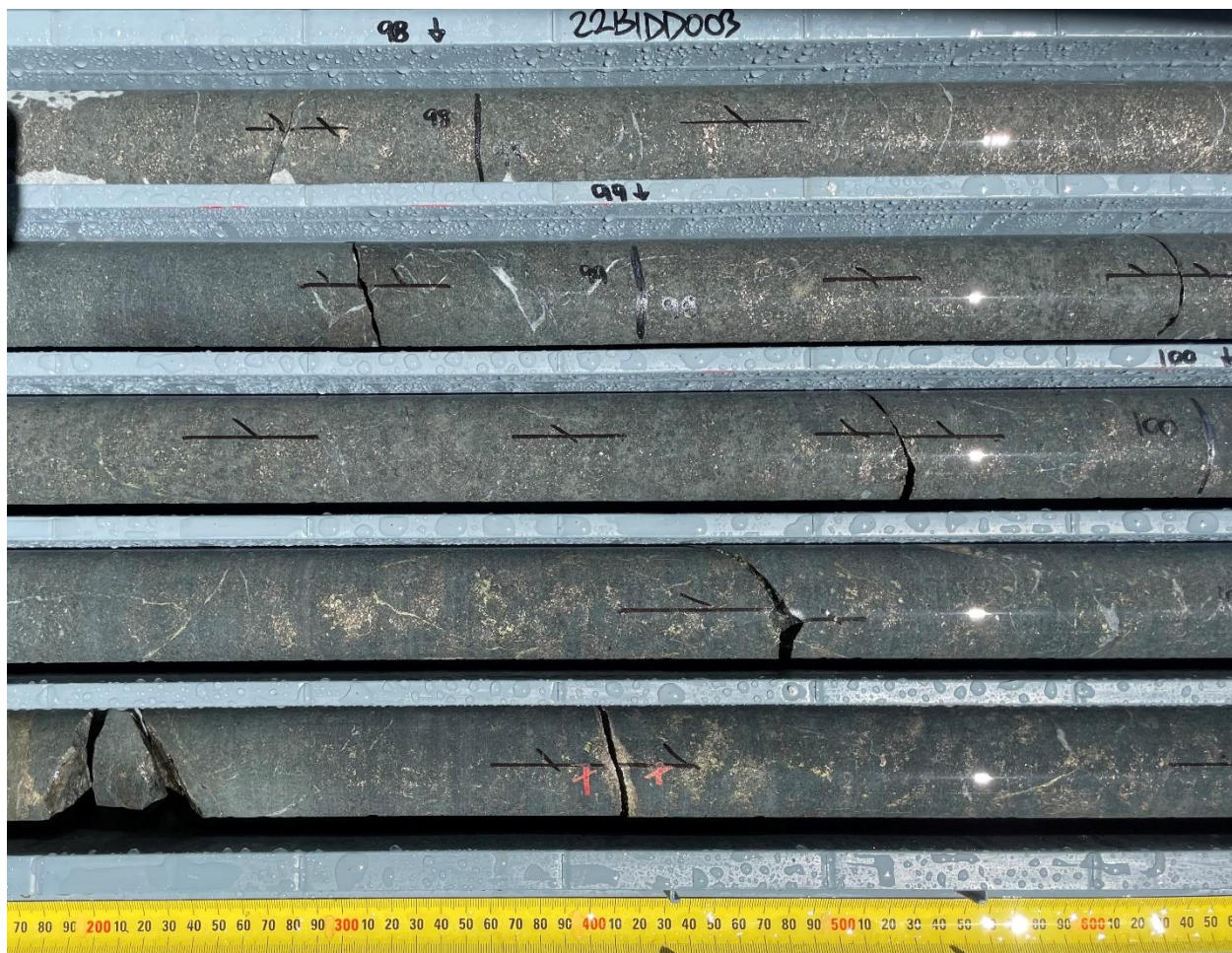
Figure 5: 22B1DD003 (included in the 85.5-107.7 metre interval – NQ core 47.6mm diameter). Mineralised dolerite with fine-grained disseminated pyrrhotite and chalcopyrite. Within a 22.2 metre zone of sulphide mineralisation. 1
