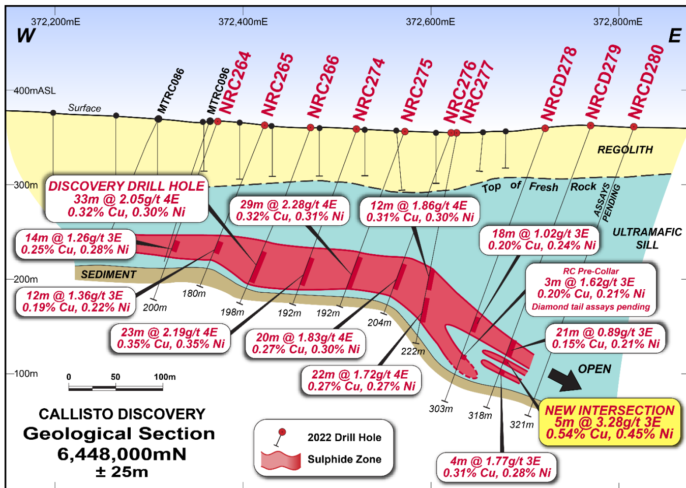
Figure 2 — Callisto geological interpretation section 6,448,000. Diamond core drill holes NRCD278, NRCD279 and NRCD280 are on the eastern side of the section (right hand side). The underlying sediment flattens at depth in drill holes NRCD279 and NRCD280. Assays are reported for NRCD279 with the new high-grade intersection highlighted in yellow. Assays are pending for diamond core tails of NRCD278 and NRCD280. RC drill holes NRC266, NRC274, and NRC275, have been twinned with diamond core holes for metallurgical test work. See Appendix 2 for drill hole collar details.
