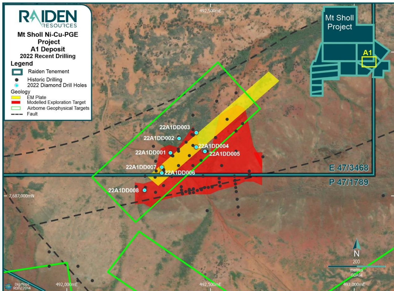
Figure 5: Mt Sholl A1 Deposit area with 2022 planned/drilled (blue dots) & historic hole locations over interpreted geology (black dots) and JORC Exploration target 3 (red).
