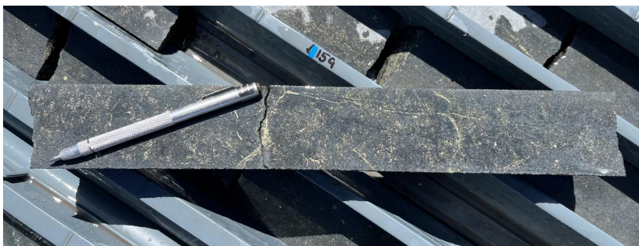
Figure 1: 22A1DD003 (156 - 165 metre interval – NQ core 47.6mm diameter). Strongly mineralised dolerite with fine-grained disseminated pyrrhotite-chalcopyrite mineralisation, within a 20.8 metre zone of sulphide mineralisation. 1
