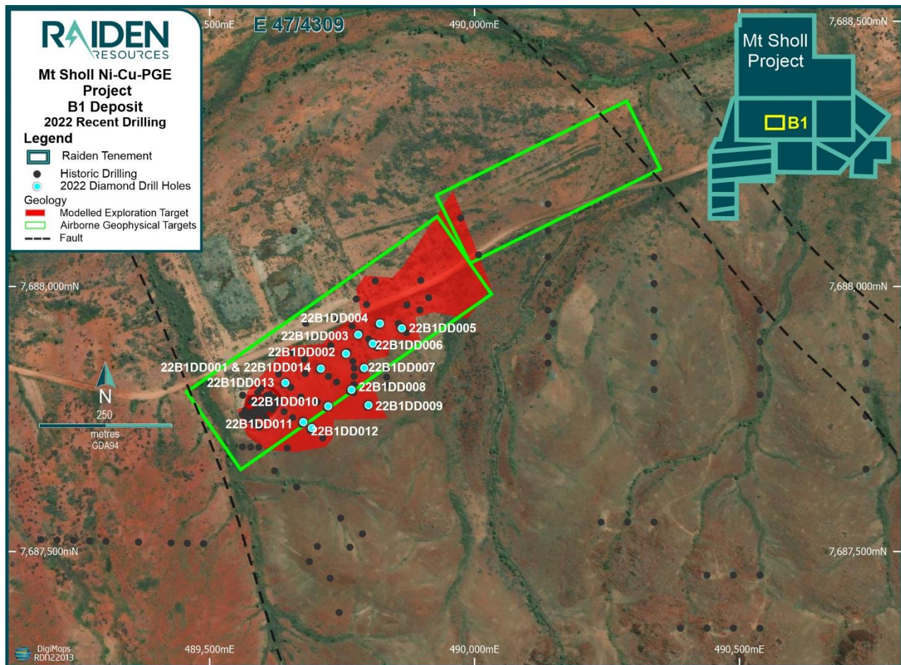
Figure 6: Mt Sholl B1 Deposit area with 2022 planned/drilled (blue dots) & historic hole locations over interpreted geology (black dots) and JORC Exploration target 3 (red).
