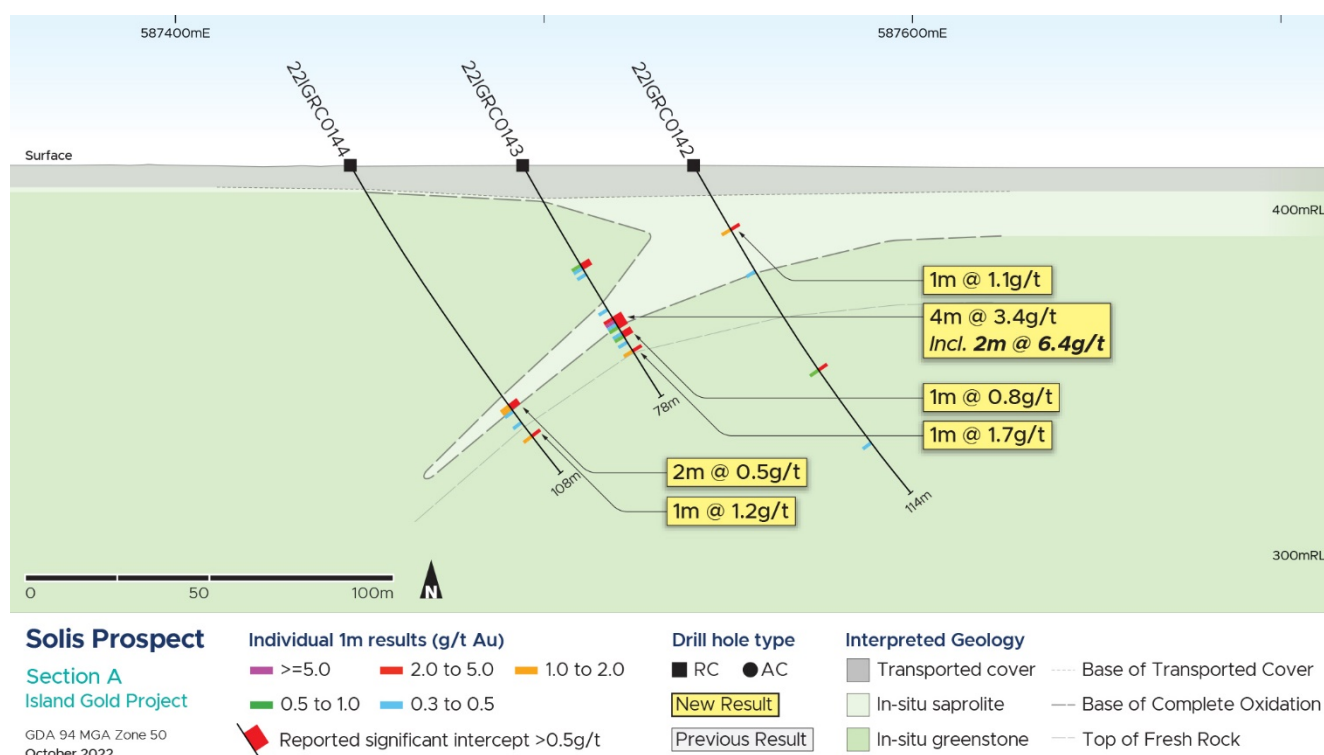
Figure 3: Solis RC cross section A, see Figure 2 for section location.
