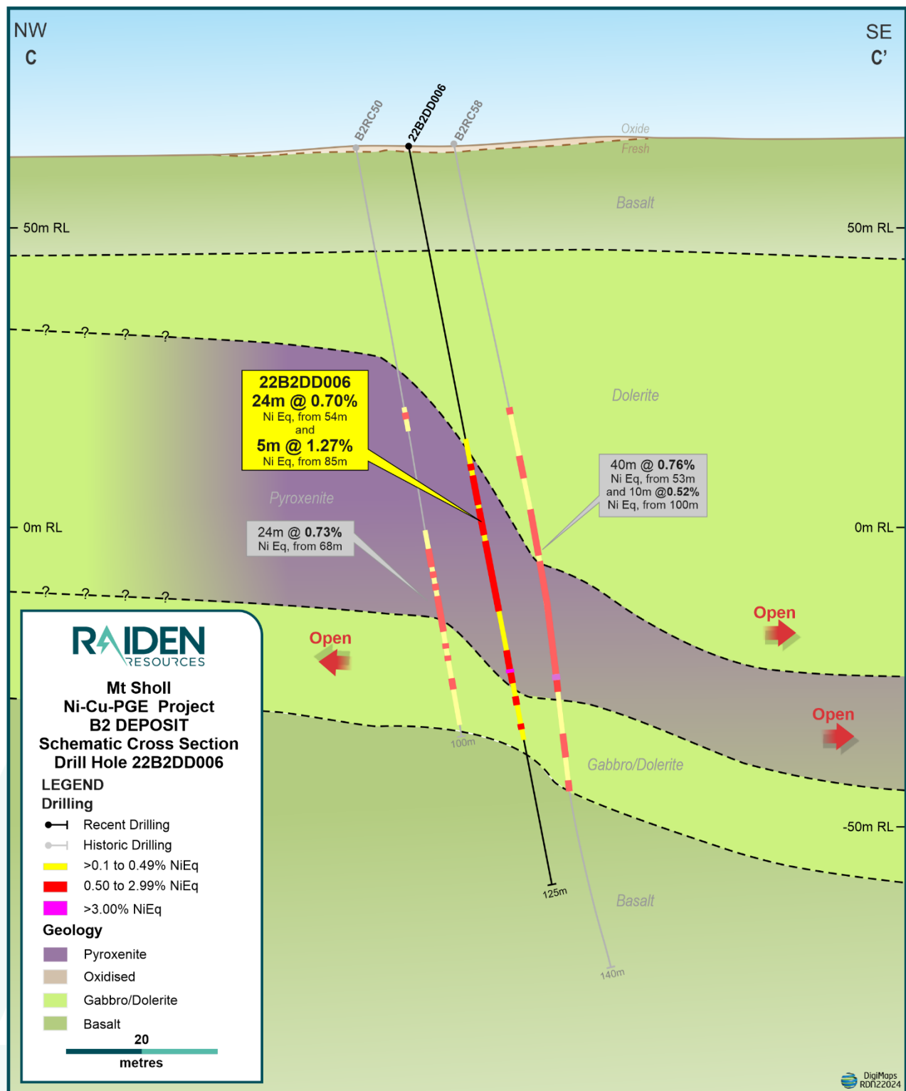
Figure 3: Section C-C' with recent hole 22B2DD006 with historical intercepts.
