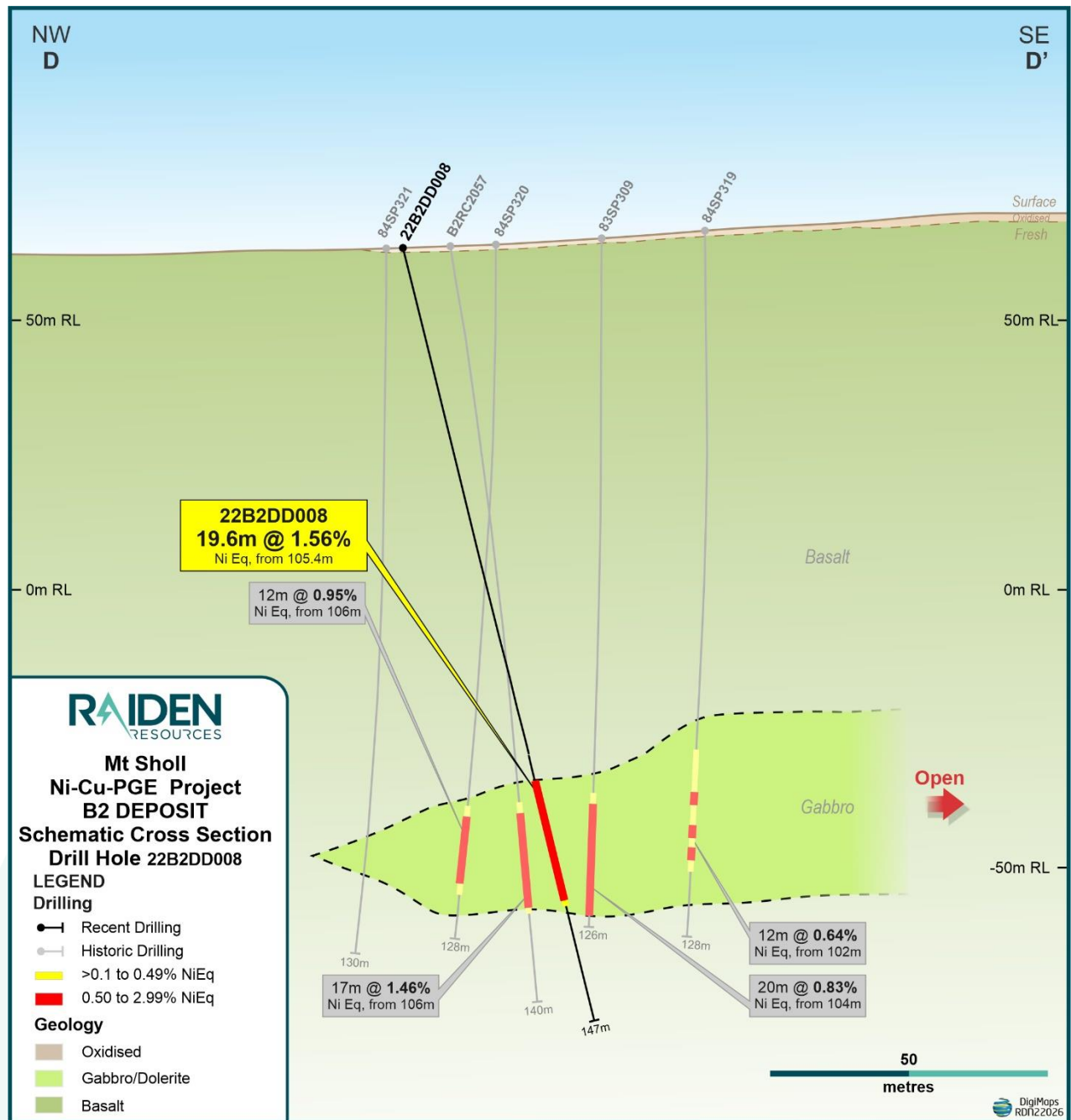
Figure 4: Section D-D' with recent hole 22B2DD008 with historical intercepts.
