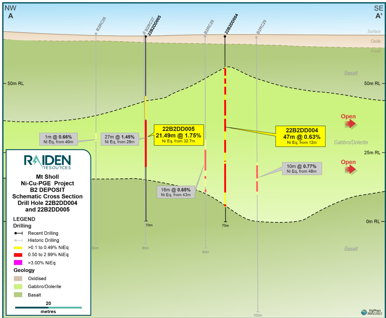
Figure 1: Section A-A' with recent holes 22B2DD004 & 22B2DD005 with historical intercepts.
