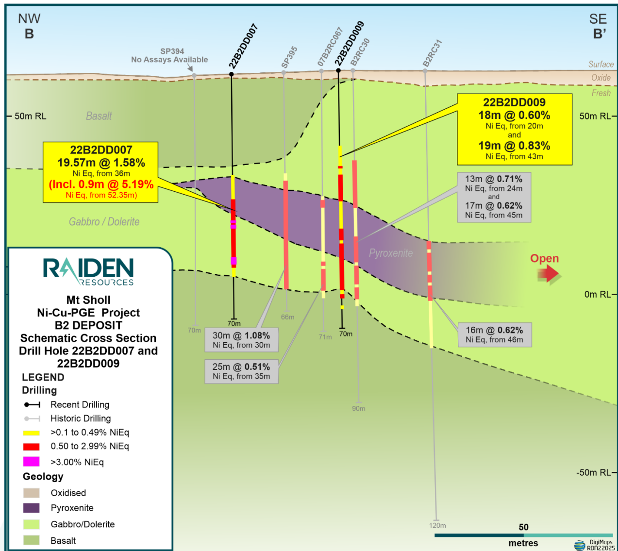
Figure 2: Section B-B' with recent holes 22B2DD007 & 22B2DD009 with historical intercepts.
