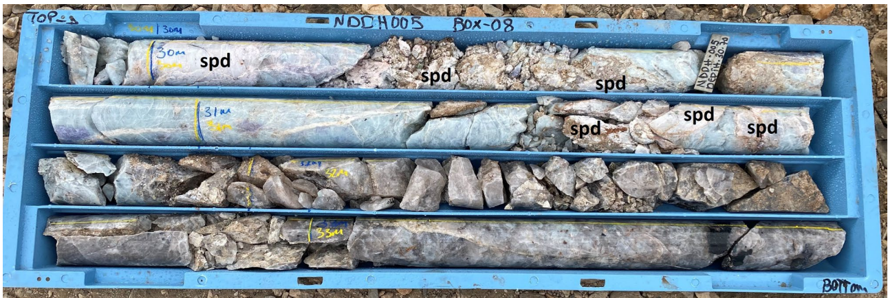
Figure 14: NDDH005 Core-tray #8. Spodumene labelled spd. Pale blue = albite (variety cleavelandite), purple = lepidolite, grey = quartz
