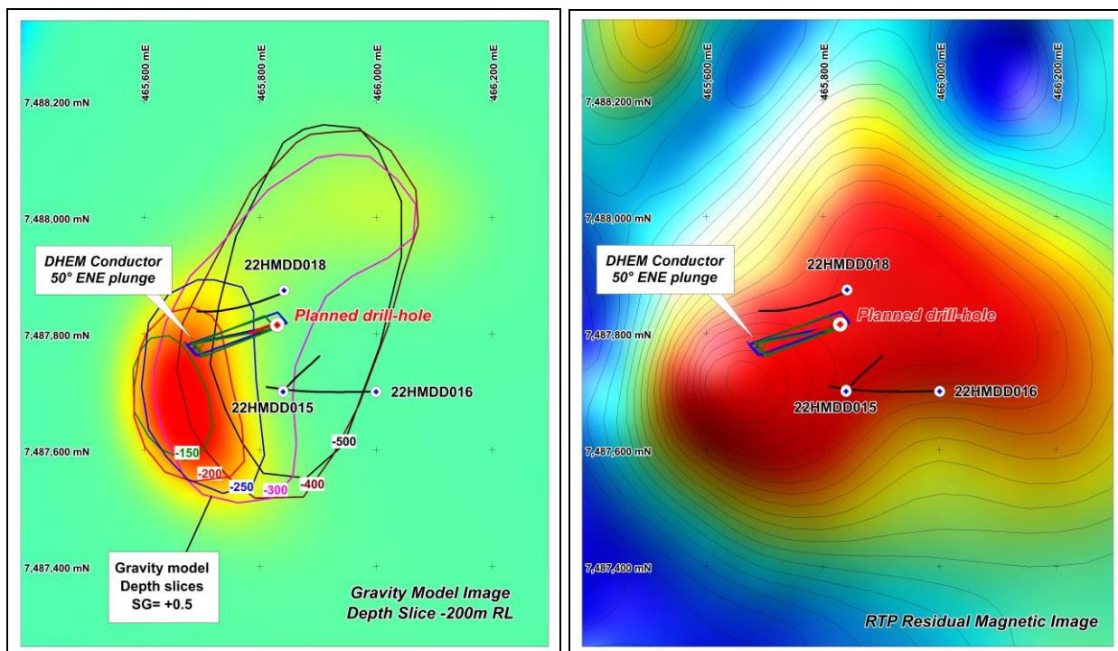
Figure 1: Hamilton North gravity & magnetics showing location of drill-holes and DHEM conductor
