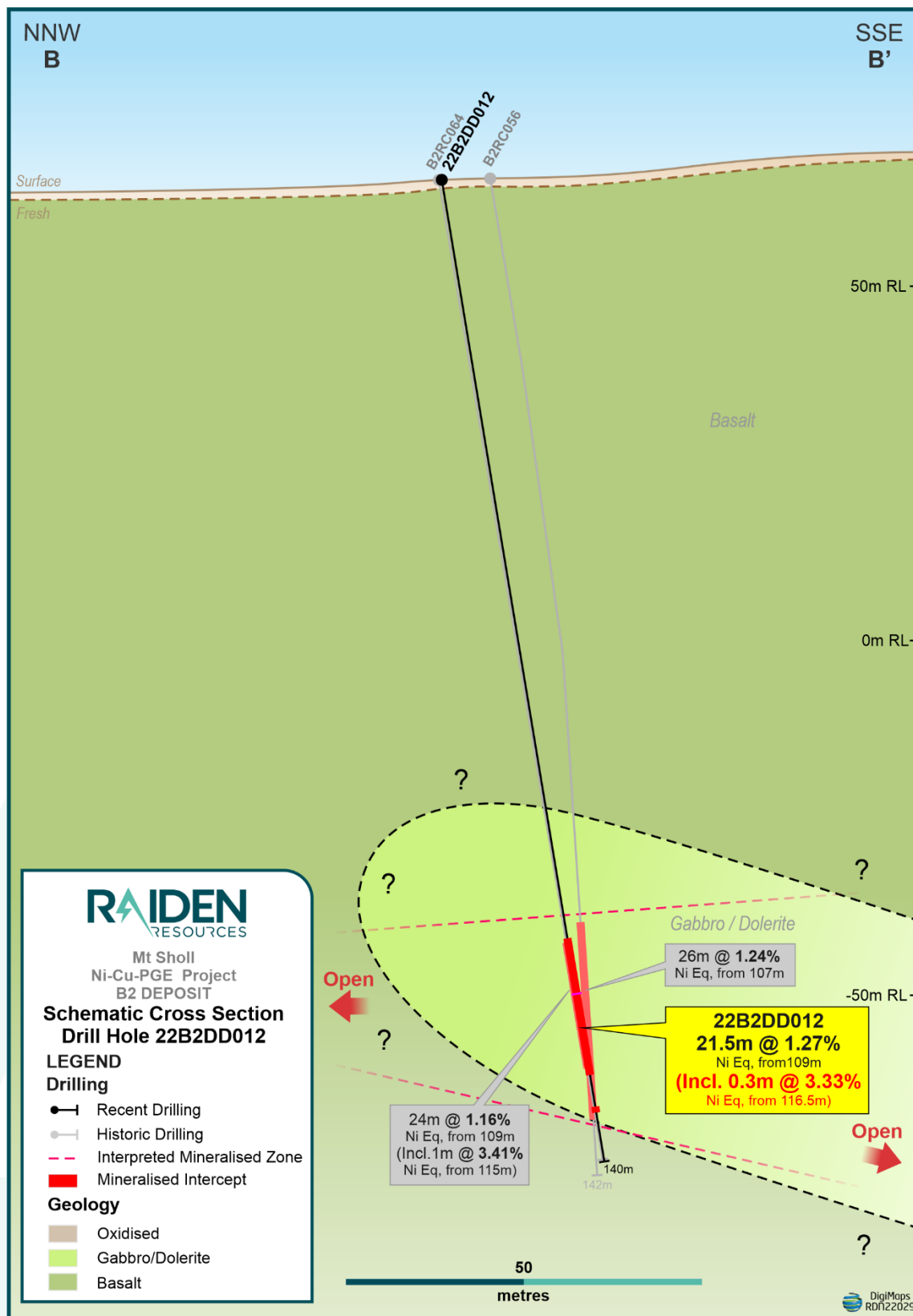
Figure 6: Section B-B' with recent hole 22B2DD012 with historical intercepts.
