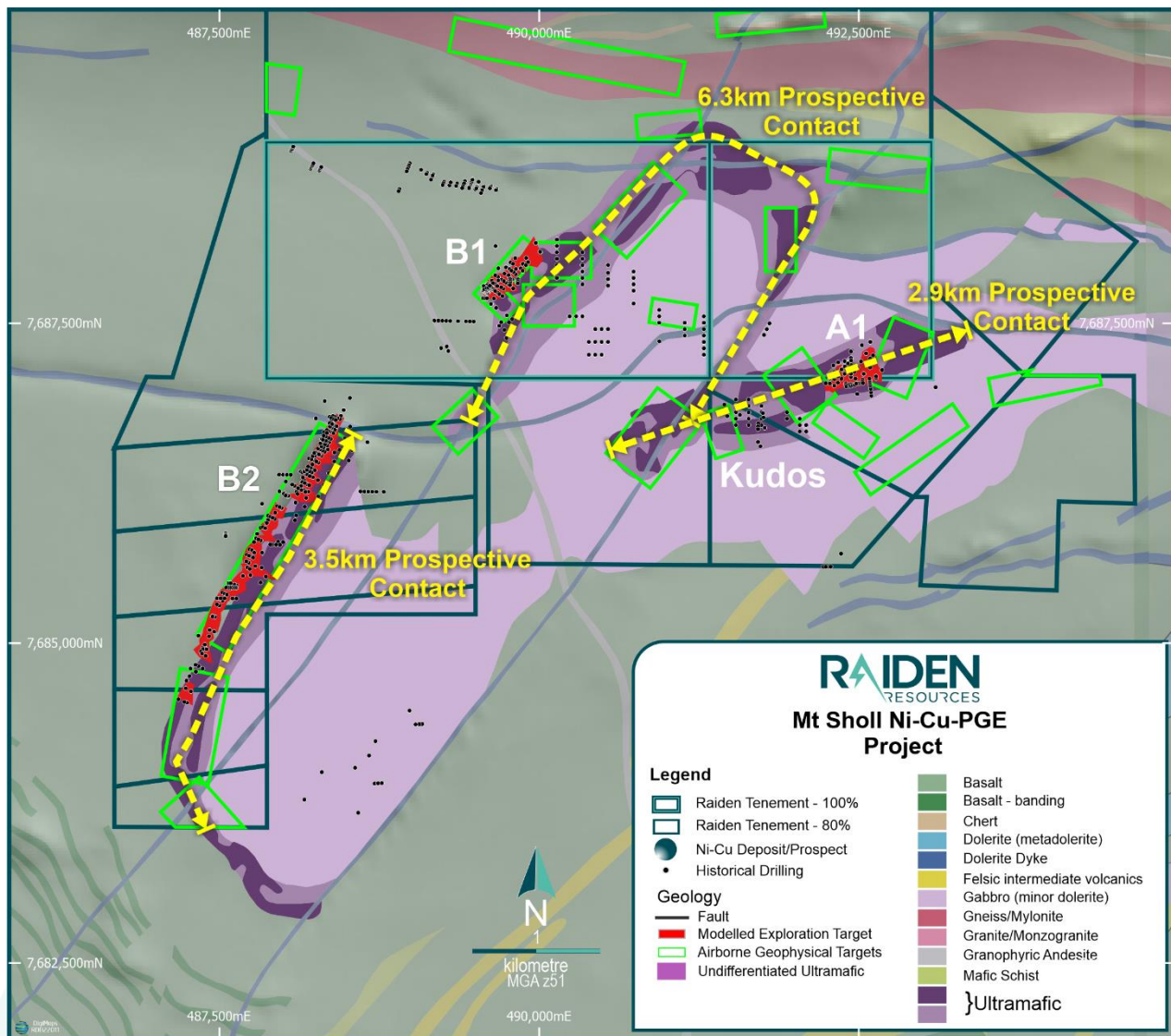
Figure 3: Mt Sholl Project area with Prospective Contact zones, drill hole locations over interpreted geology, JORC Exploration target 3 (red) and EM targets (green).
