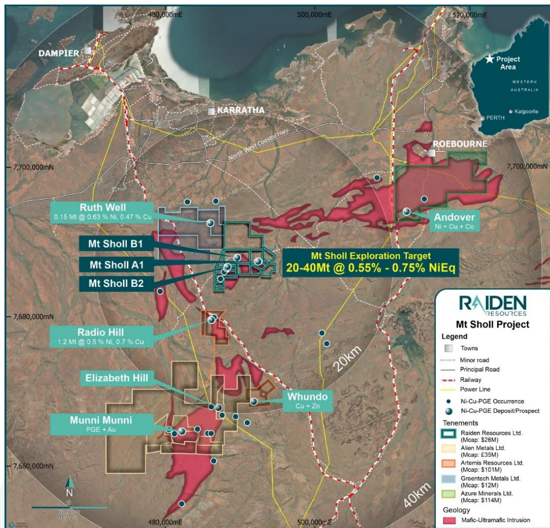
Figure 9: Mt Sholl Project in relation to key infrastructure and nearby JORC (2012) Resources. 3,4,5
