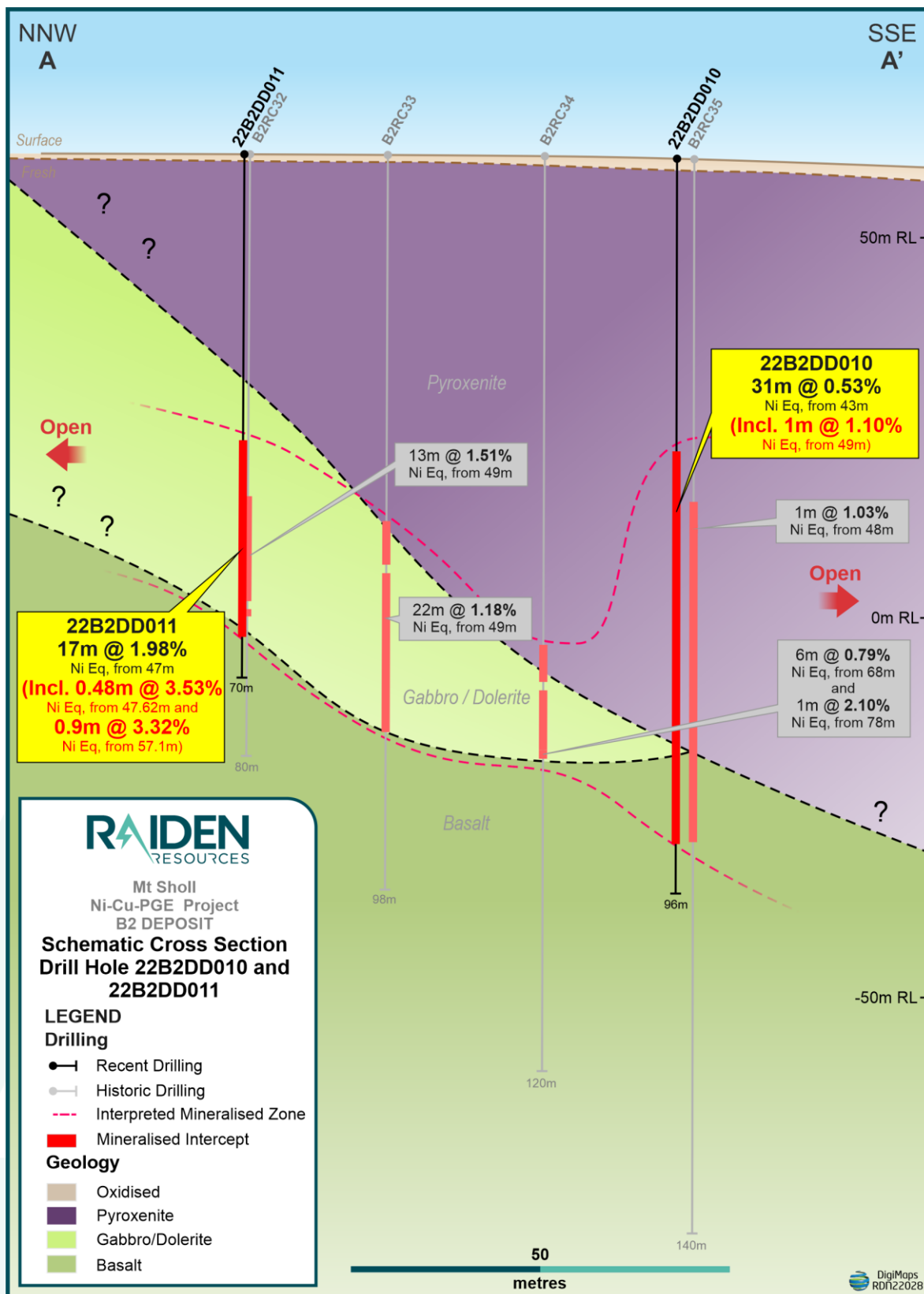
Figure 5: Section A-A' with recent holes 22B2DD010 & 22B2DD011 with historical intercepts.
