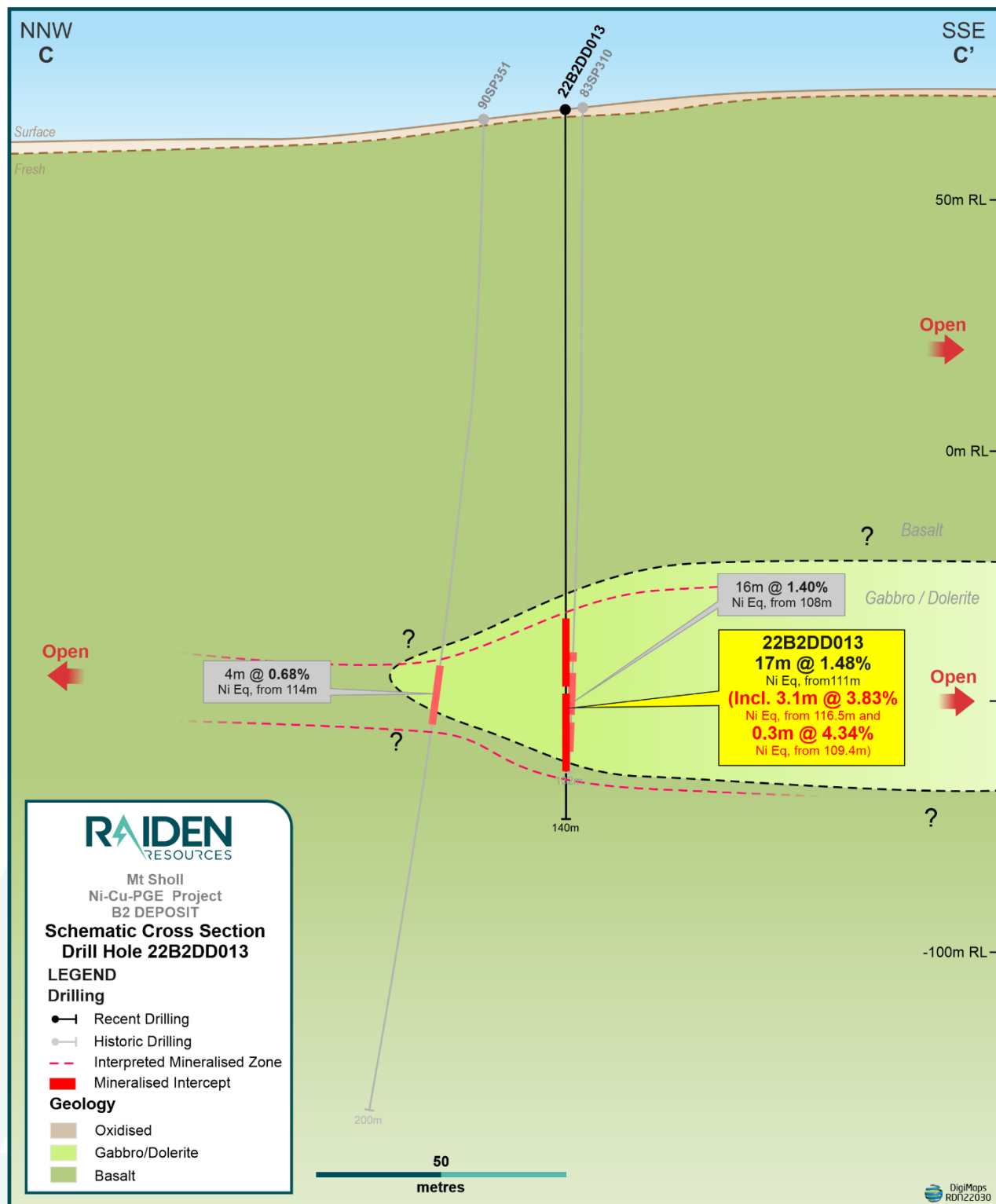
Figure 4: Section C-C' with recent hole 22B2DD0013 with historical intercepts.
