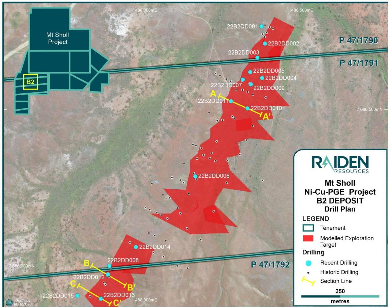
Figure 7: Mt Sholl B2 Deposit area with recent drill locations and section lines over JORC Exploration target. 3
